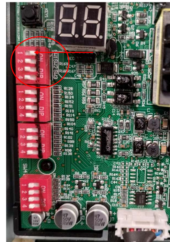
Indoor Unit
