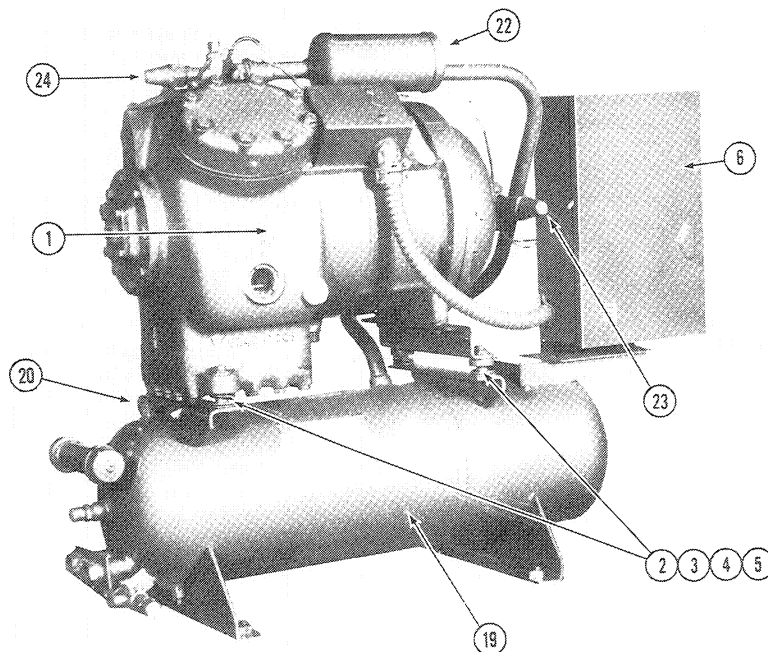
Typical 6 Cylinder Water-Cooled Condensing Unit (07DA210, Three-Phase Illustrated)
