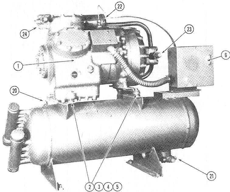
Typical 4 Cylinder Water-Cooled Condensing Unit (07DA106, Three-Phase Illustrated)
