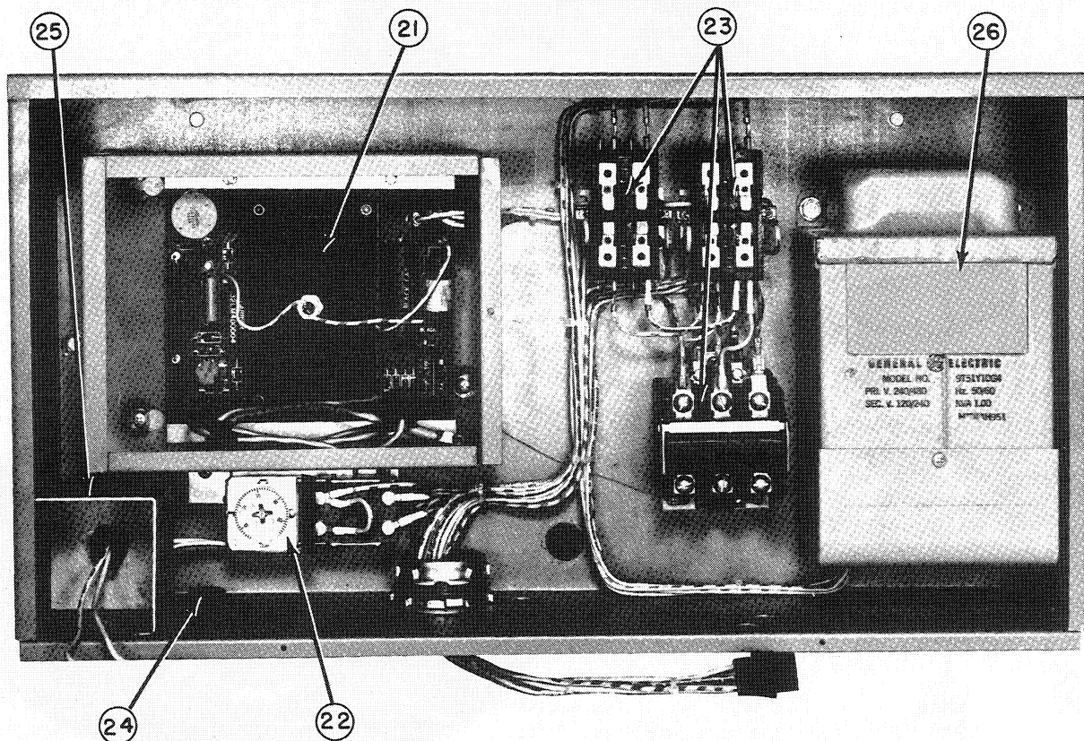
Control Box 09DA
