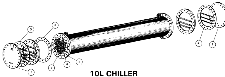
10L CHILLER
