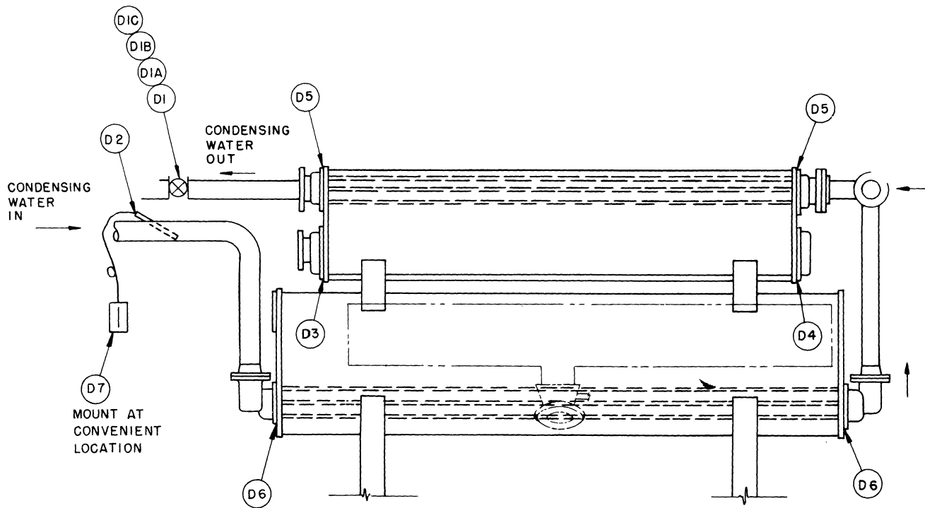
CONDENSING WATER CIRCUIT
