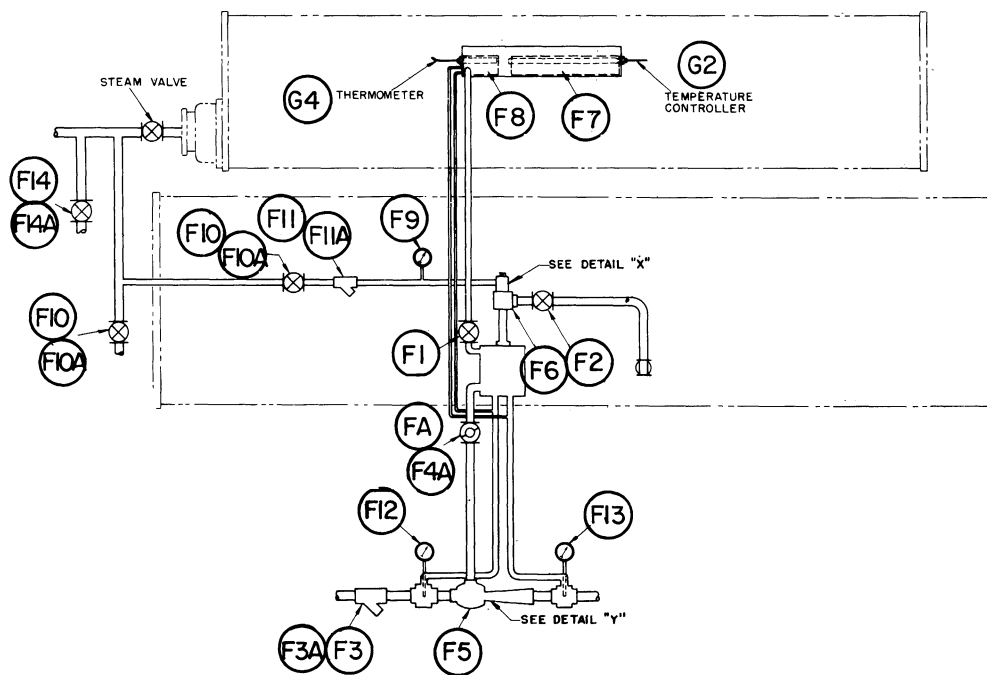
PURGE CIRCUIT
