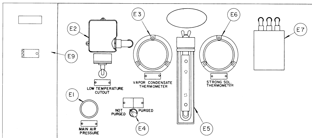
Control Panel for 16C12 - 16C13 Machines
