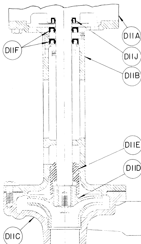
Jet Purge Pump (Allis Chalmers Keyed Shaft)
