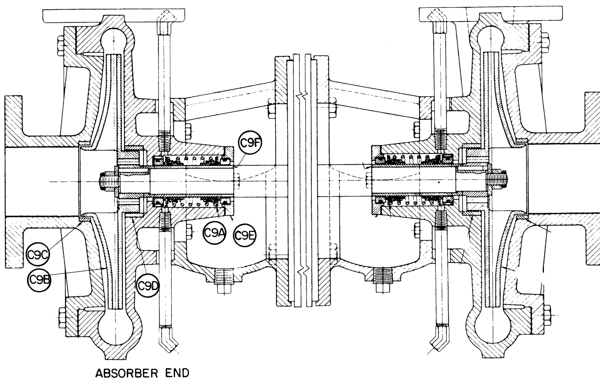
Double Solution Pump — Open
