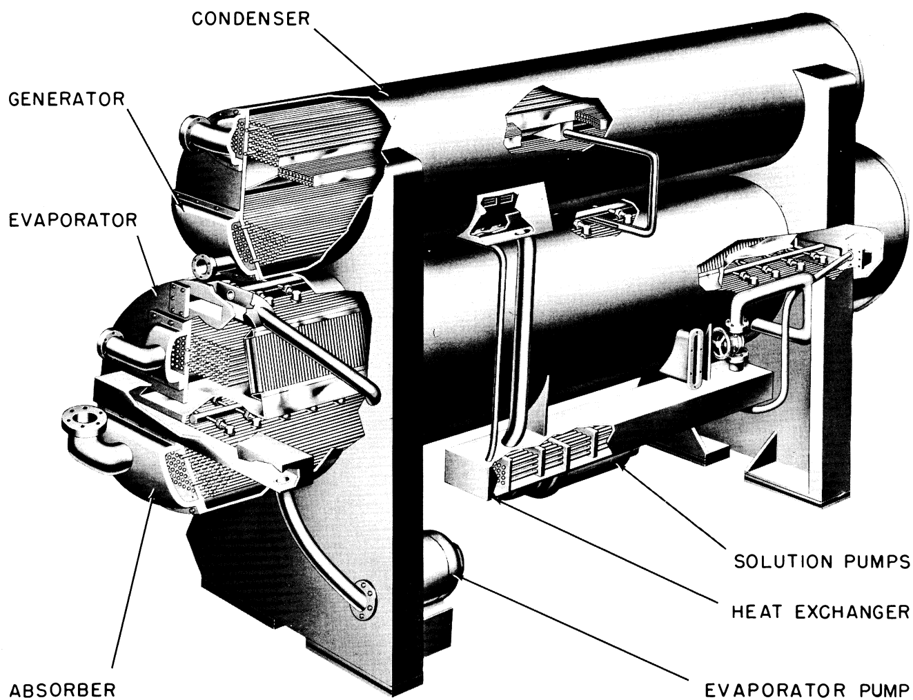
Cutaway of Typical 16C Absorption Machine
