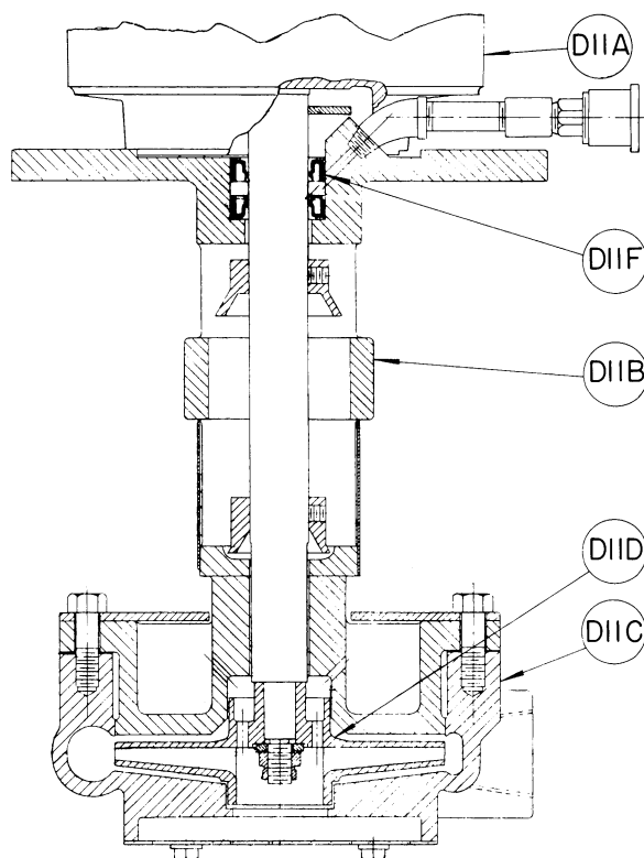
JET PURGE PUMP (BUFFALO KEYED SHAFT)
