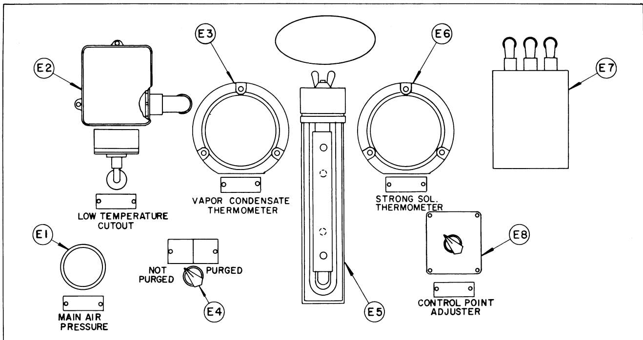
Control Panel for 16C2 - 16C11 Machines
