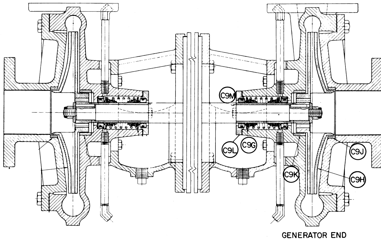
Double Solution Pump — Open
