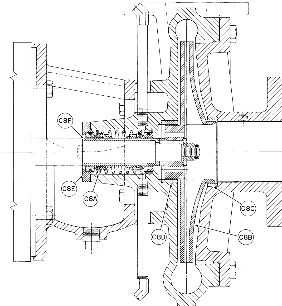
Evaporator Pump
