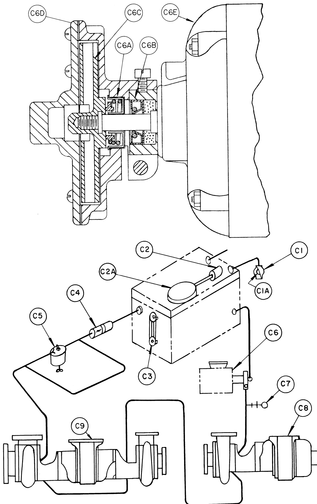
Circulating Seal Water System
