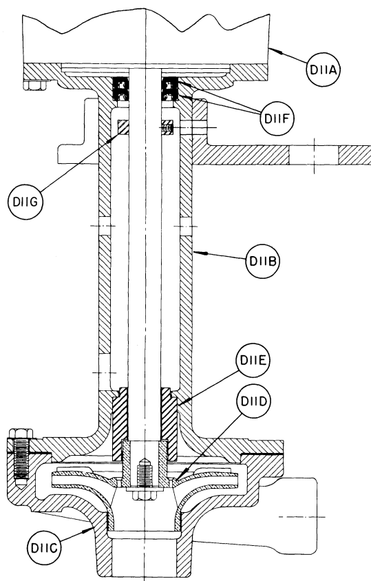
Jet Purge Pump (Allis Chalmers Keyed Shaft)
