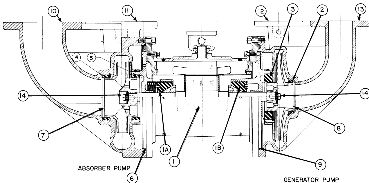
Group E — Double Solution Pump - Hermetic
