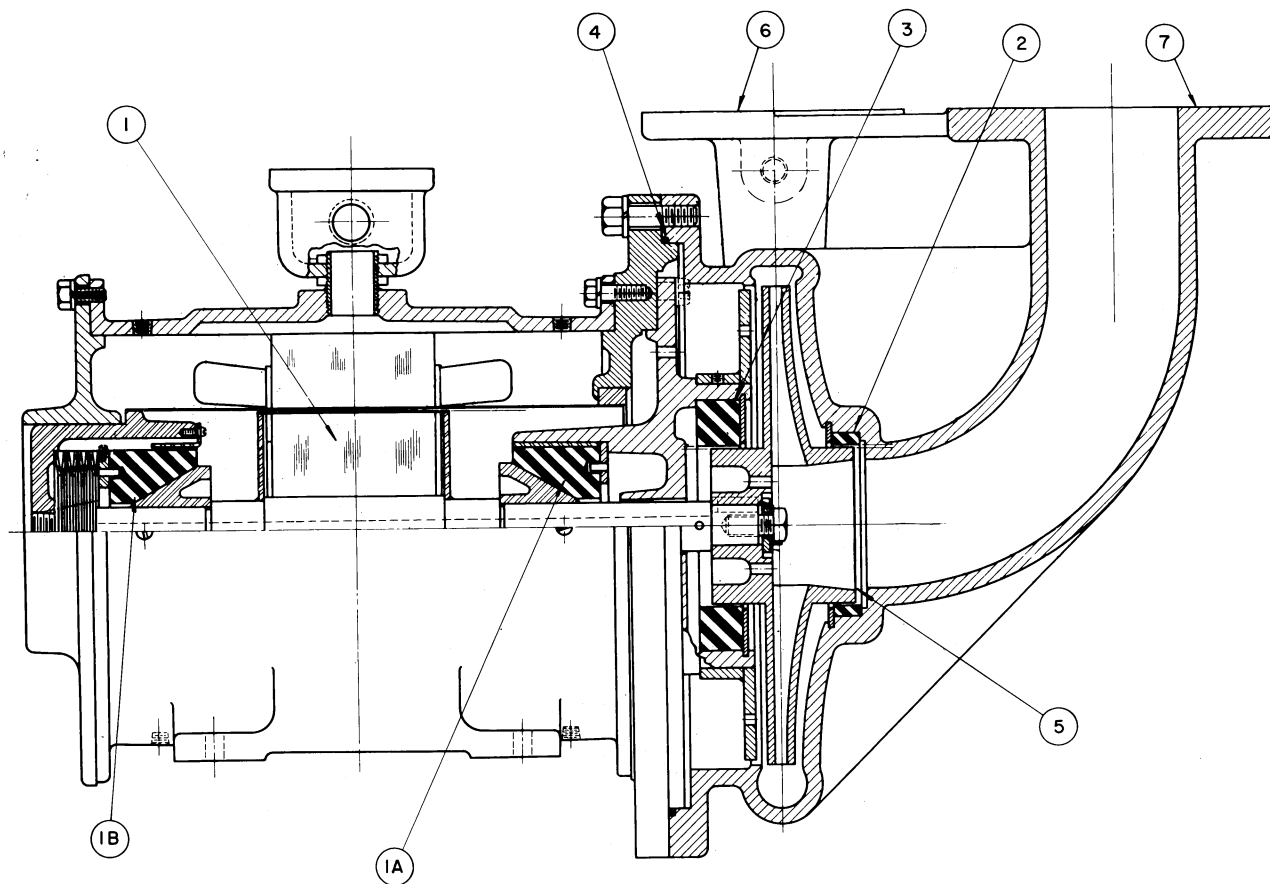
Group C and D — Refrigerant Pump - Hermetic
