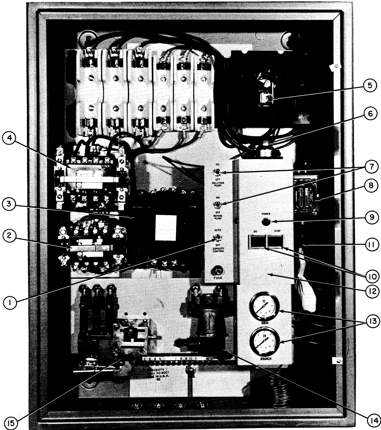
Group F — Control Center (Electronic and Pneumatic)
