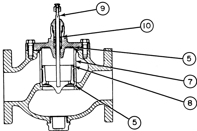
Group F - Pneumatic Steam Valve (Modified Linear and Equal Percentage Ports)
