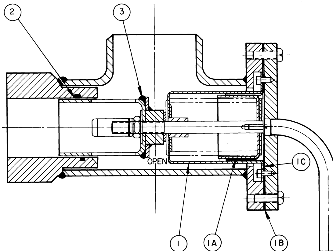
ABSORBER VALVE ASSEMBLY
