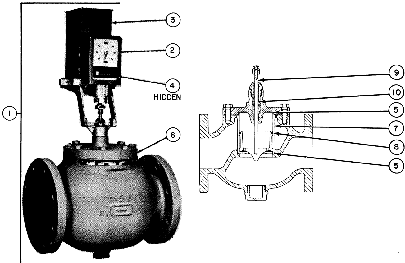
Group E-Electronic Steam Valve (Modified Linear and Equal Percentage Ports)
