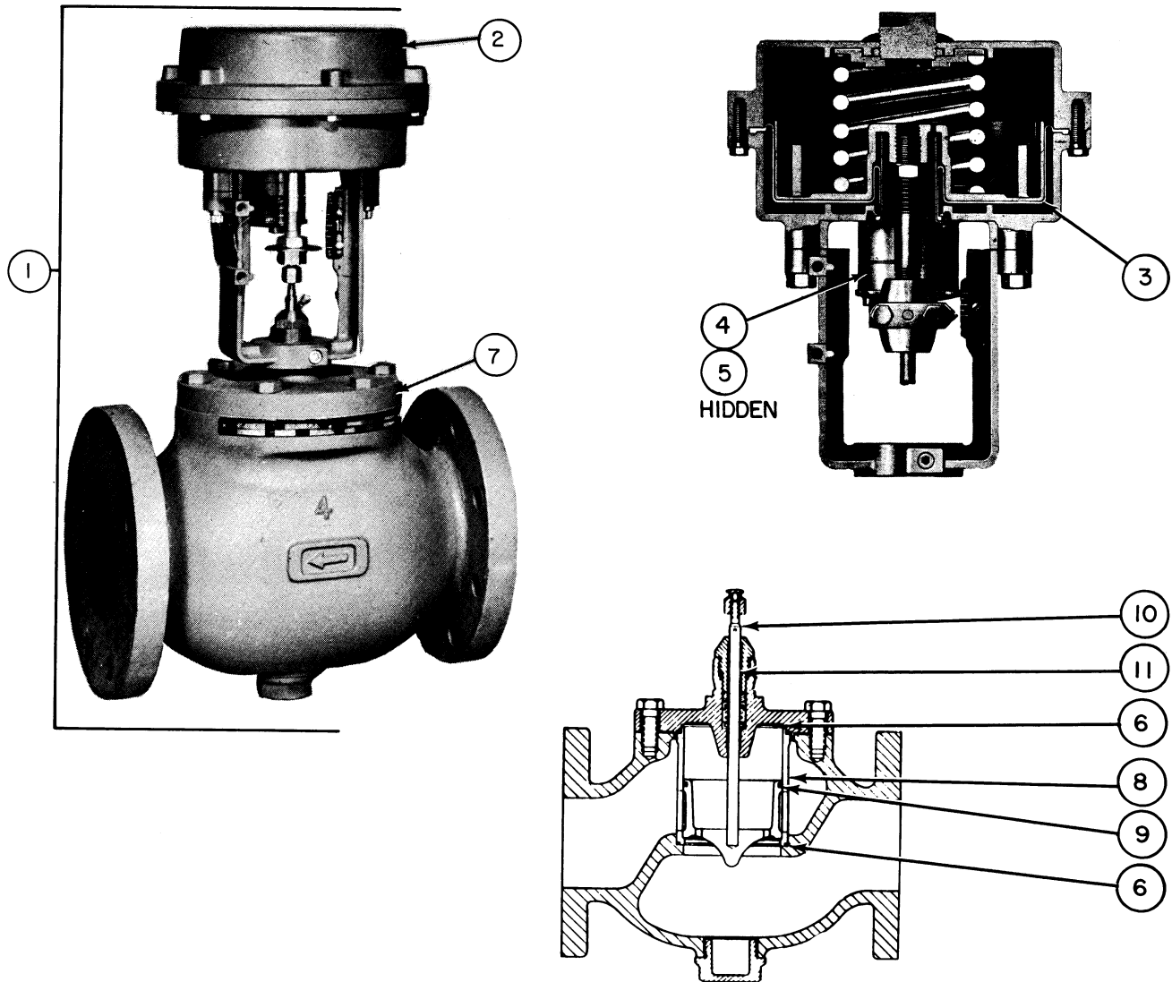
Group G-Pneumatic Steam Valve (Caged)
