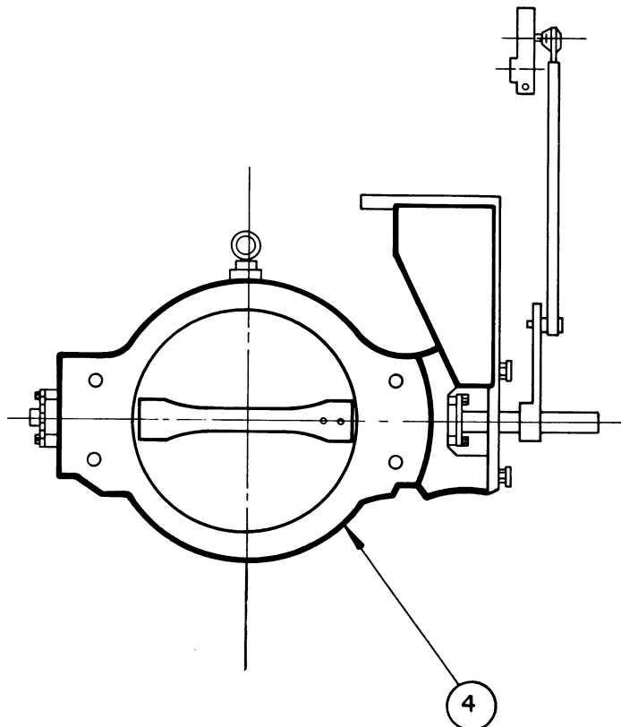
Group F-Electronic Steam Valve (Butterfly)
