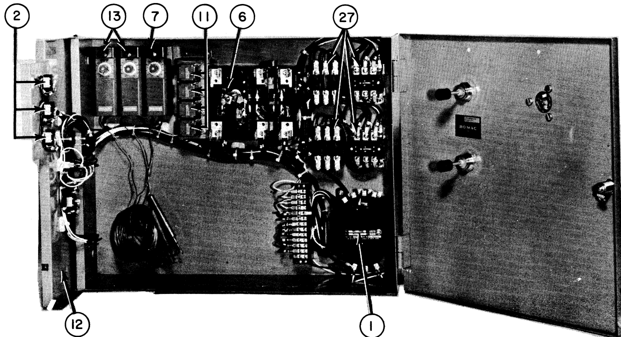
Group J-Control Panel (Electronic and Pneumatic)
