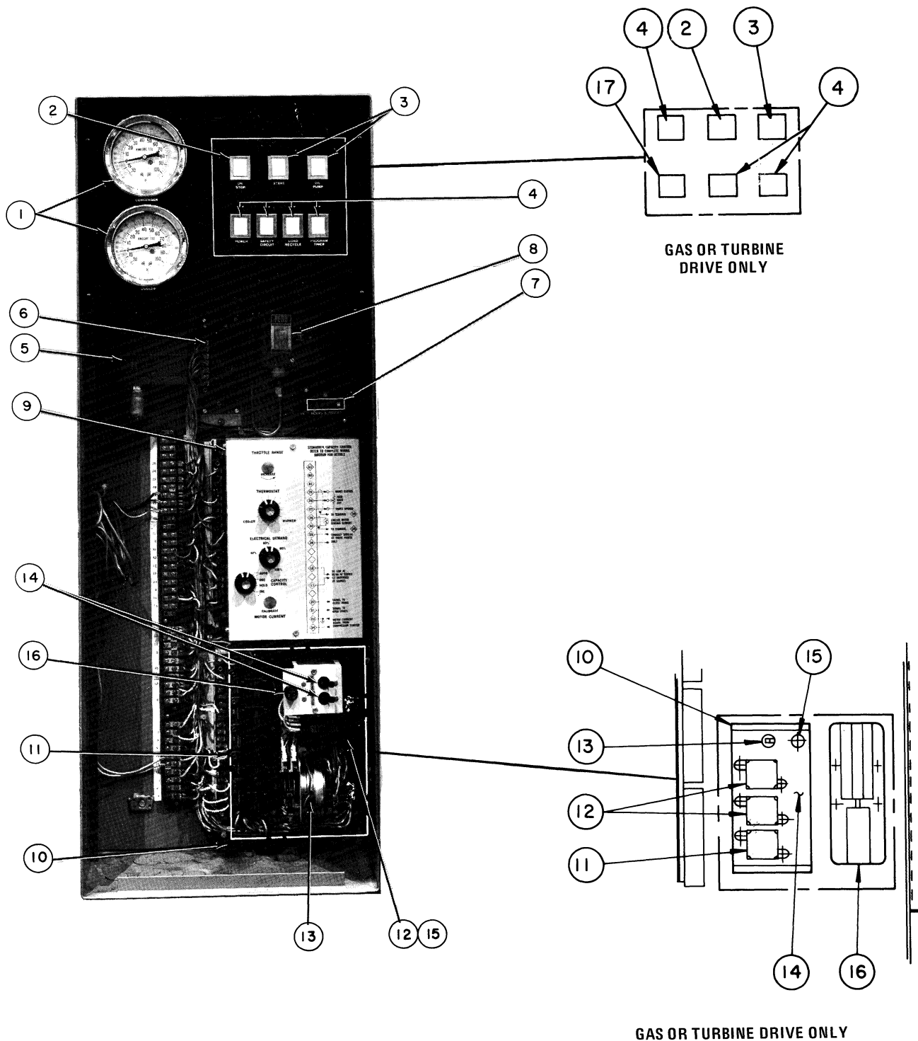
Group M — Control Panel (Electronic)
