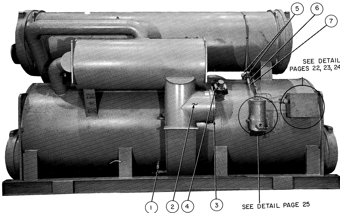
Group H — Cooler, Condenser and Economizer
