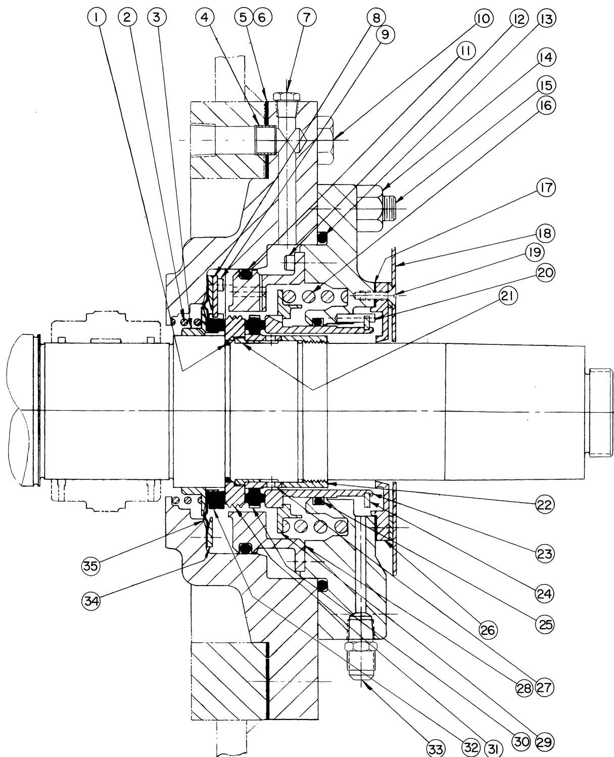
Group D — Contact Seal
