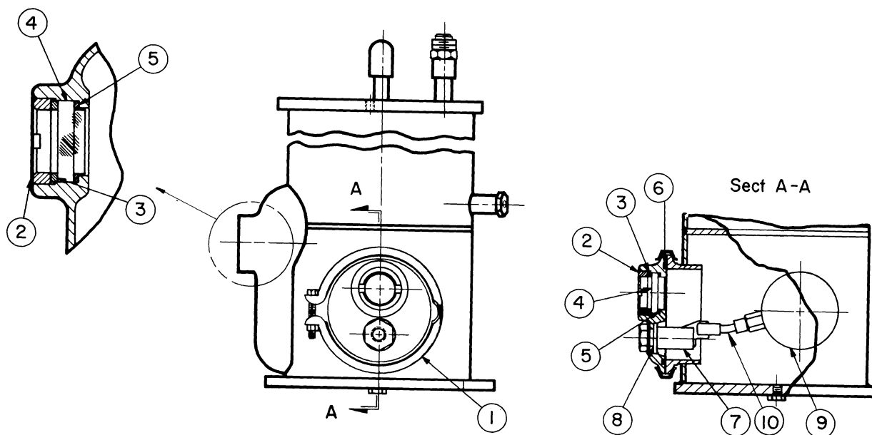
Group L — Purge Assembly
