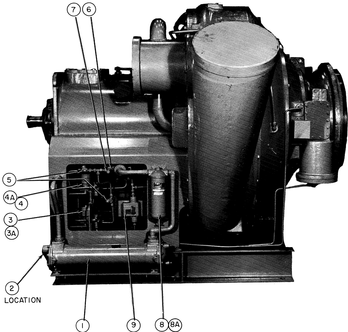
Group B — Oil Piping Arrangement
