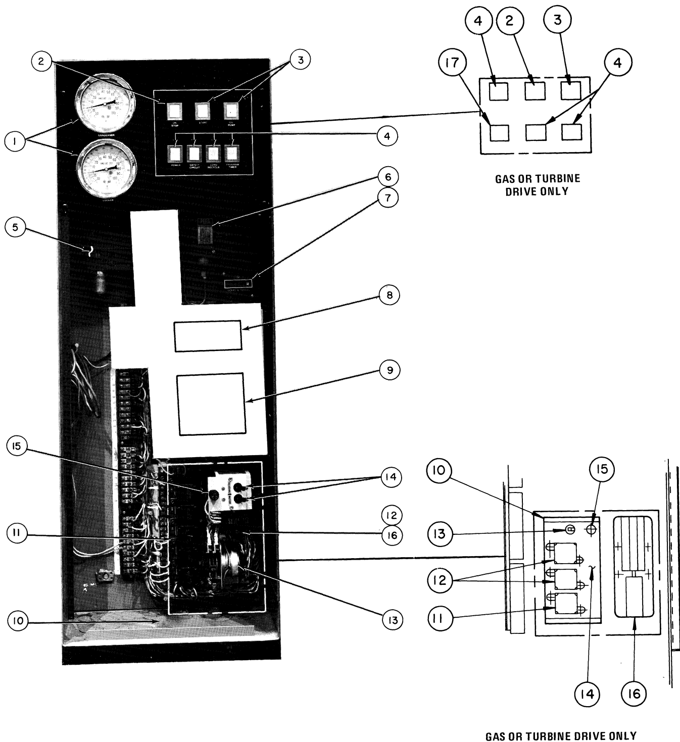
Group N – Control Panel (Pneumatic)
