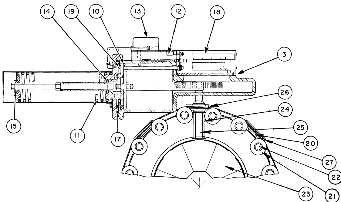
Group E — Inlet Venturi (Pneumatic,
