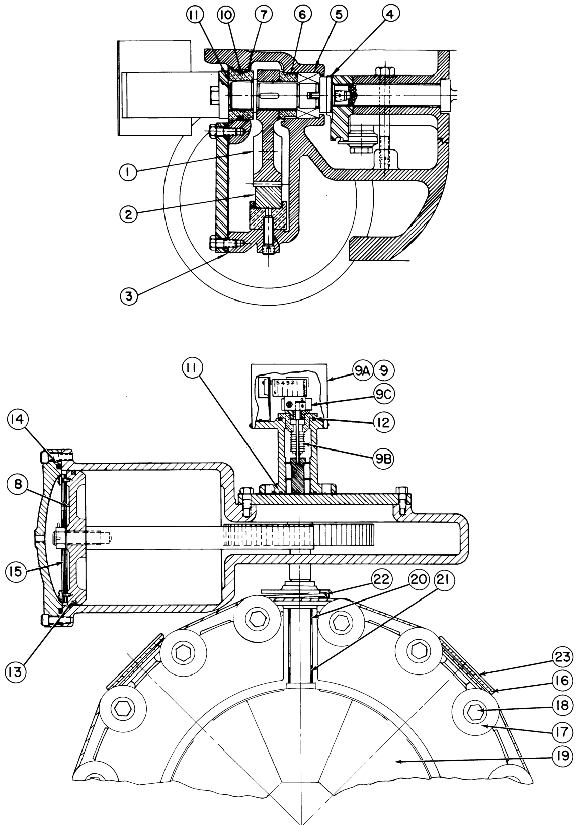
Group F – Inlet Venturi (Electronic)
