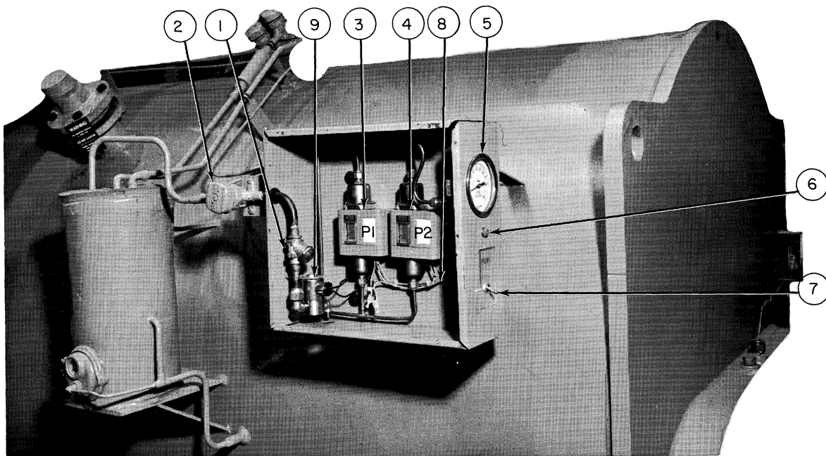
Group K — Purge Assembly Controls (R114)
