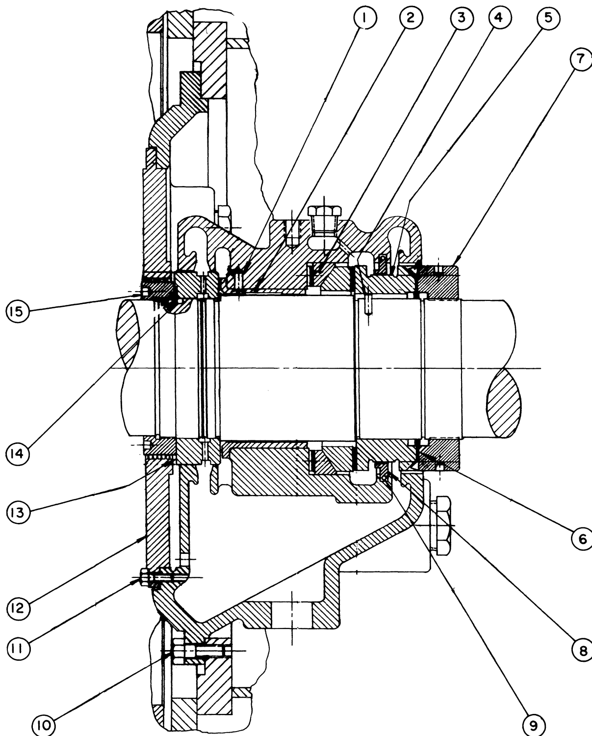
Group C — Thrust Bearing
