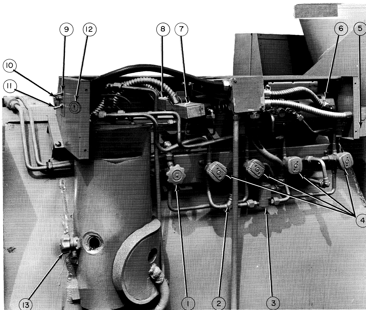
Group J — Purge Assembly Controls (R11)
