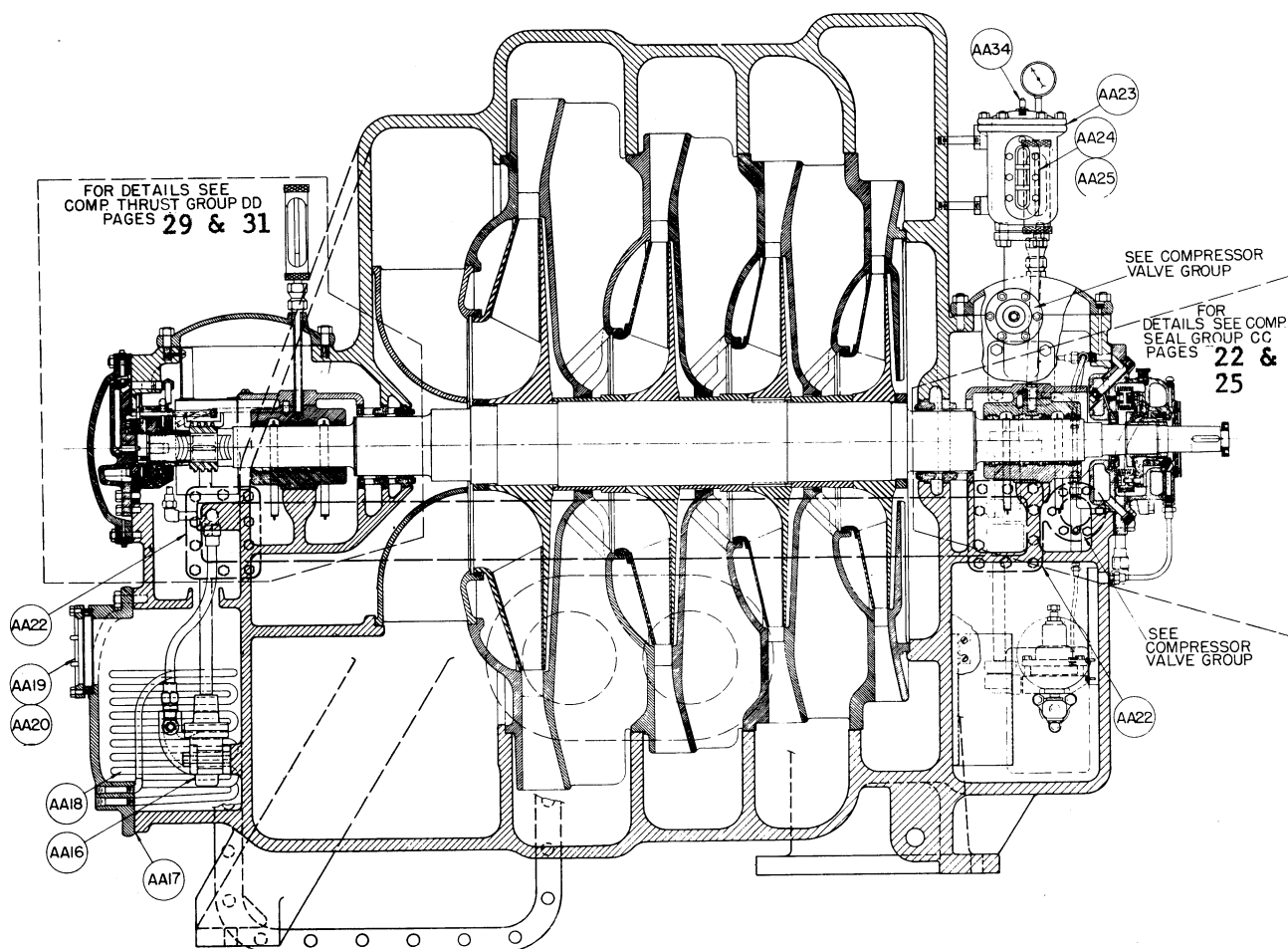
"DZ" COMPRESSOR (INTERNAL PARTS)
