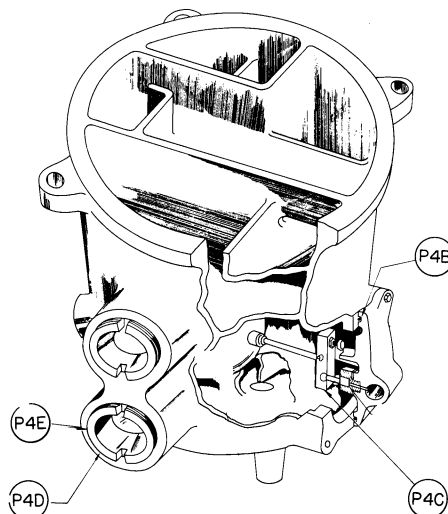
PURGE SEPARATION CHAMBER
