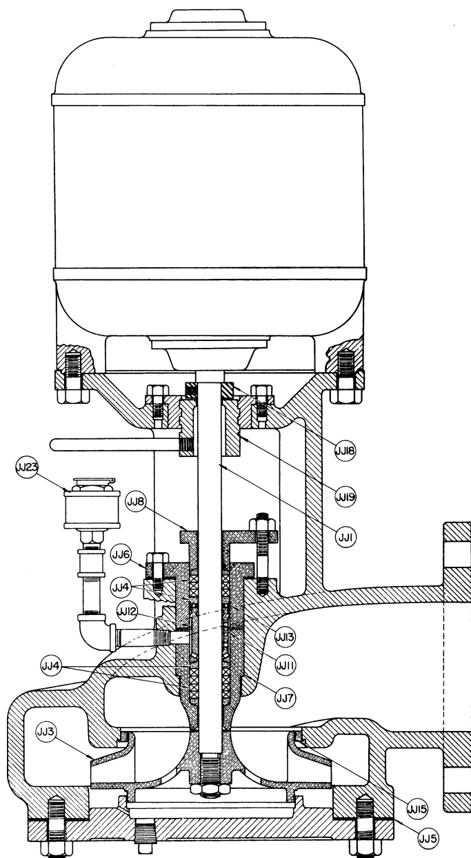
2" LIQUID PUMP
