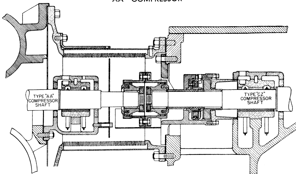
"AA" COMPRESSOR
