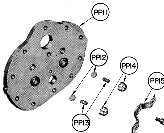
DISCHARGE VALVE PLATE ASSEMBLY
