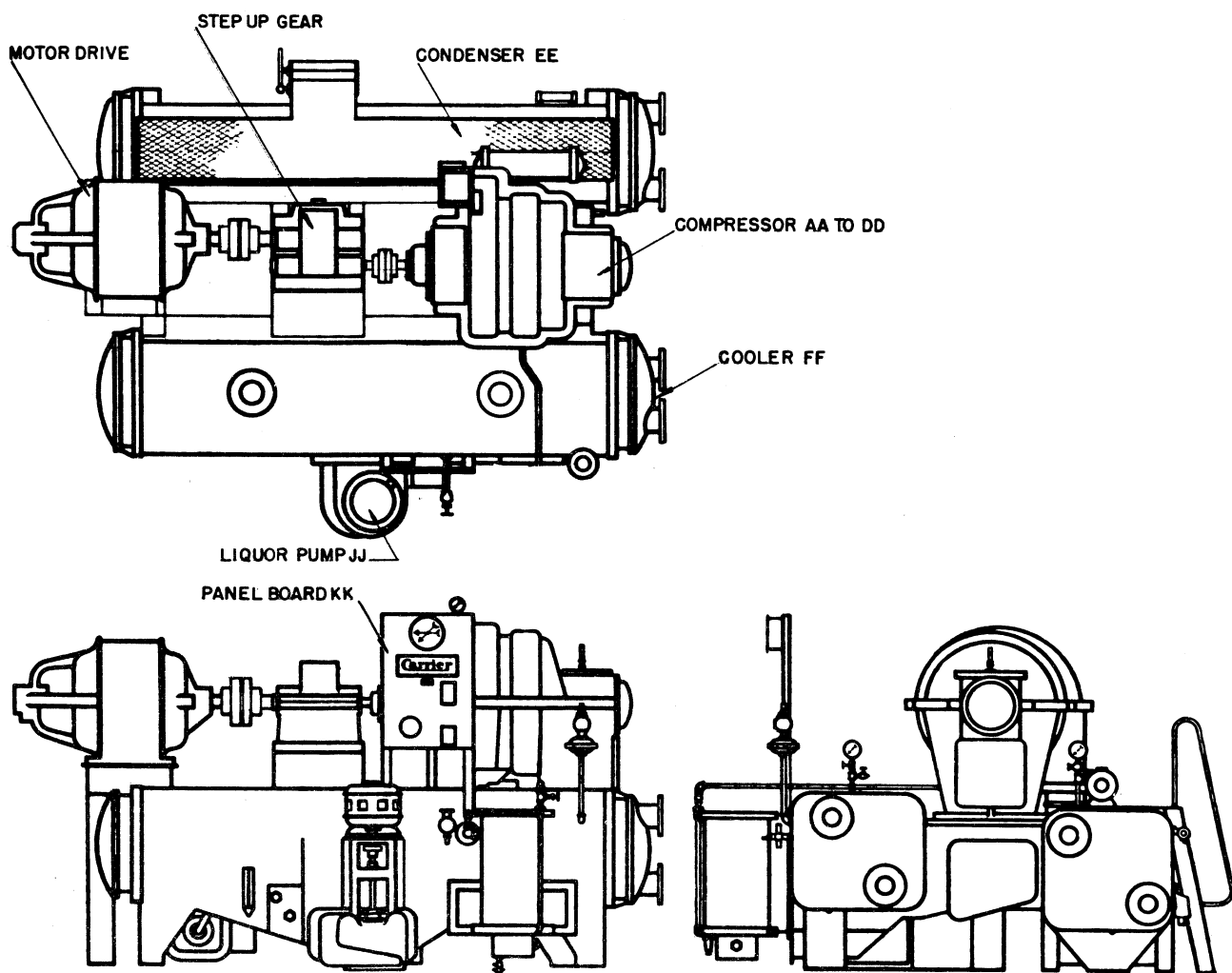
UNIT INDEXING (BY GROUPS)
