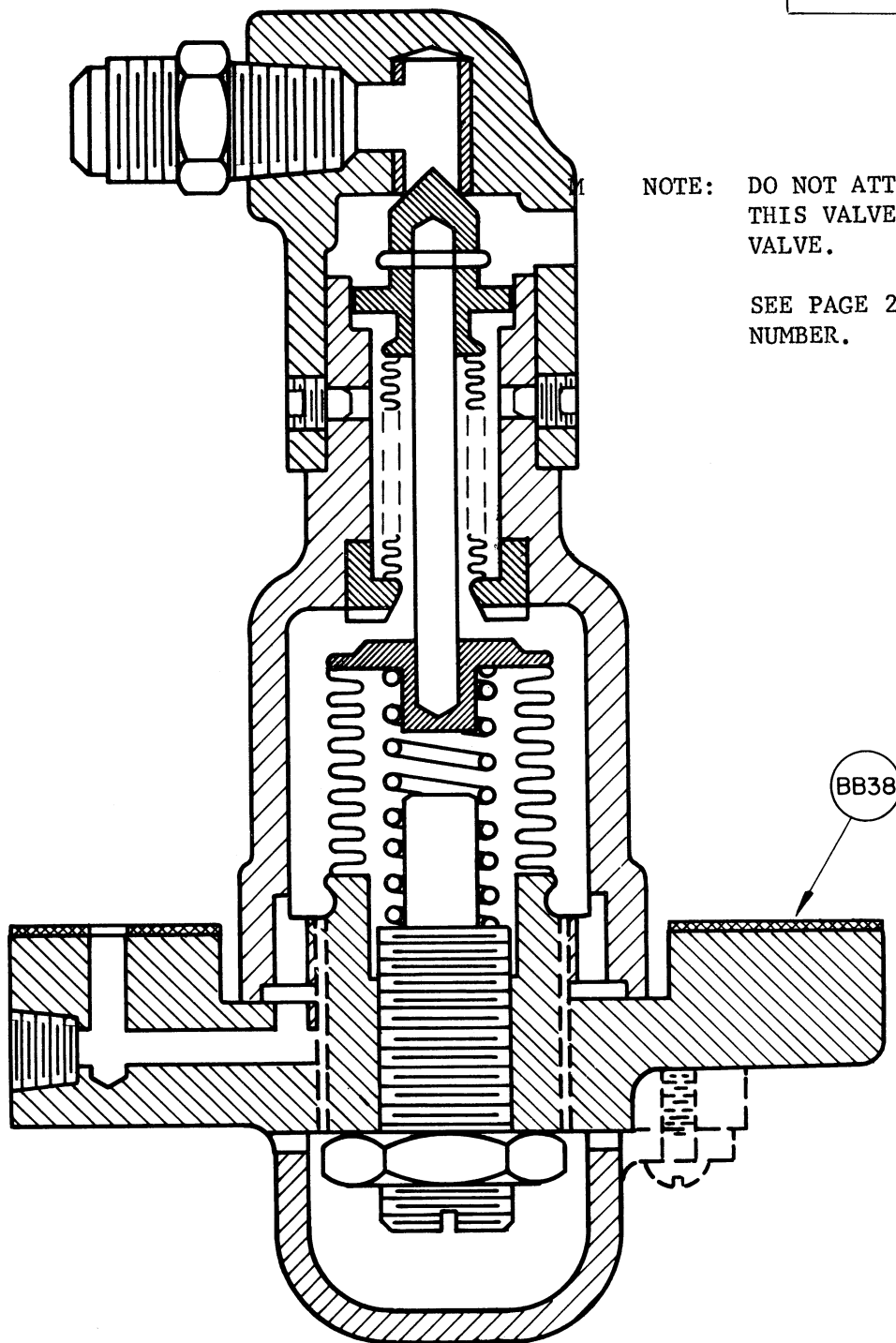
"DZ" OIL PRESSURE REGULATING VALVE
