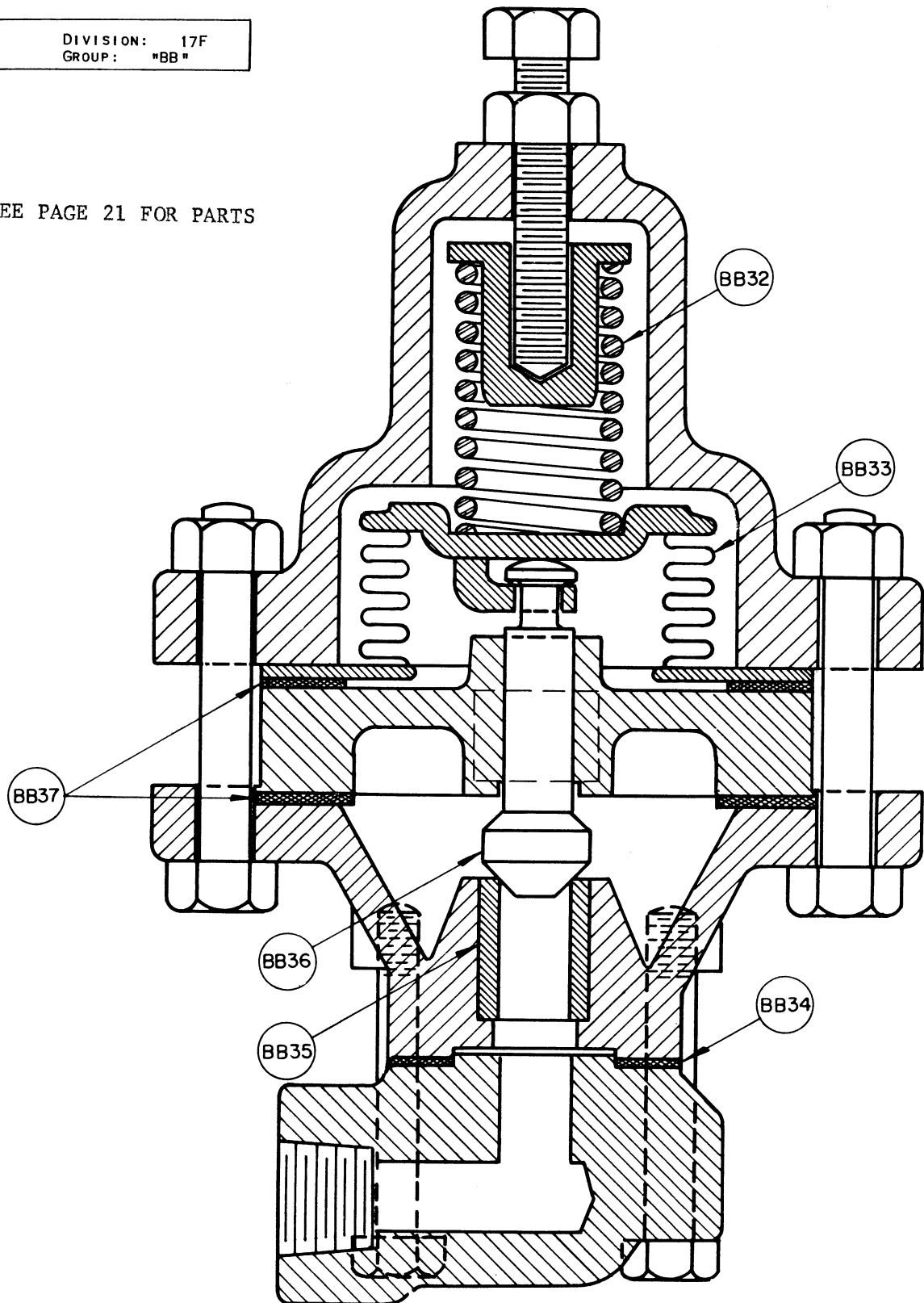
"DZ" OIL STOP VALVE
