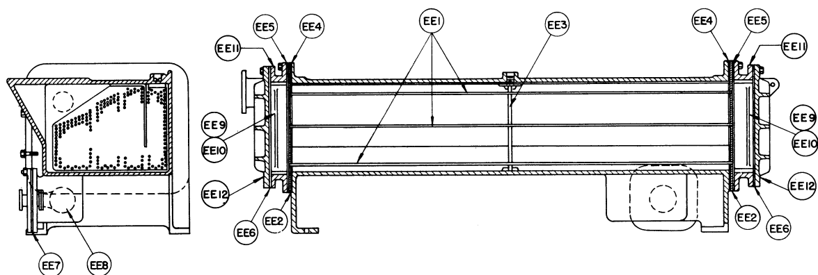
CAST IRON CONDENSERS #7 1/2 THRU #10 1/2
