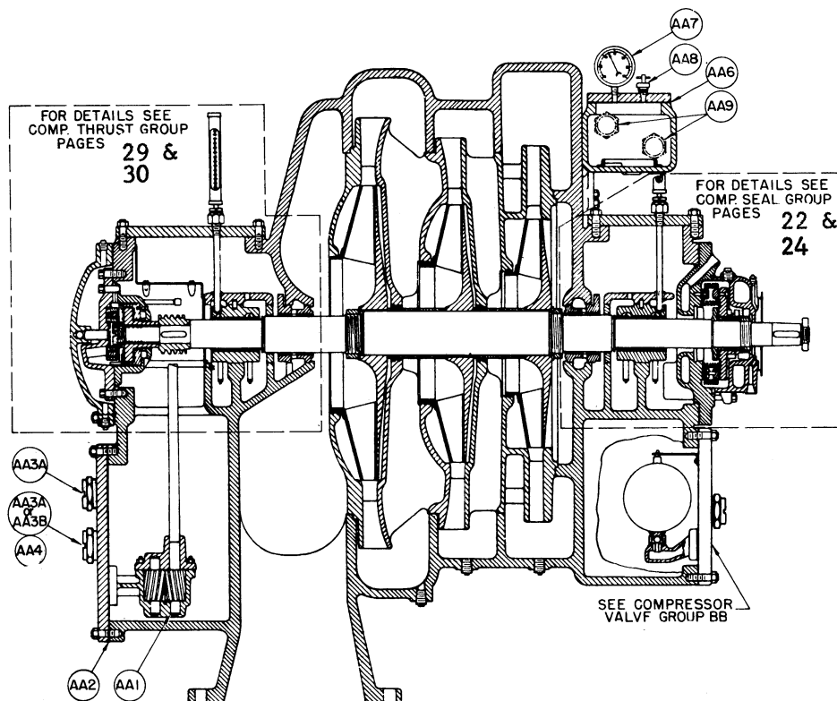
"CZ" COMPRESSOR (INTERNAL PARTS)
