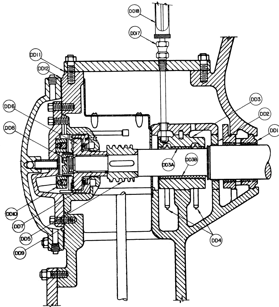
"CZ" AND "DZ" COMPRESSOR THRUST PARTS
