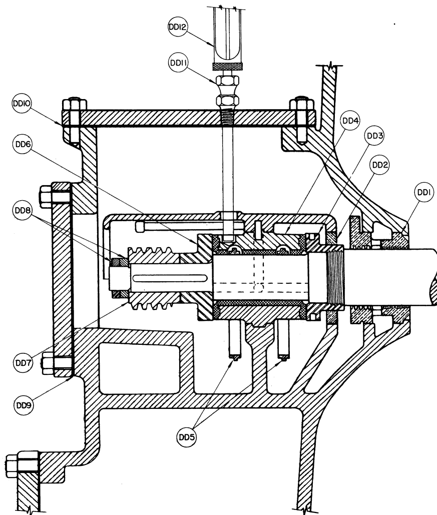
TYPE "AA" AND "BZ" COMPRESSOR THRUST END
