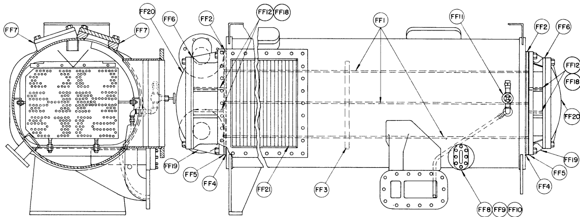
WELDED STEEL COOLER #6 1/2
