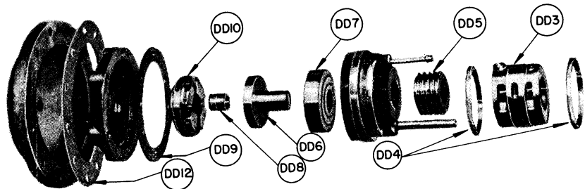
"CZ" AND "DZ" COMPRESSOR THRUST PARTS
