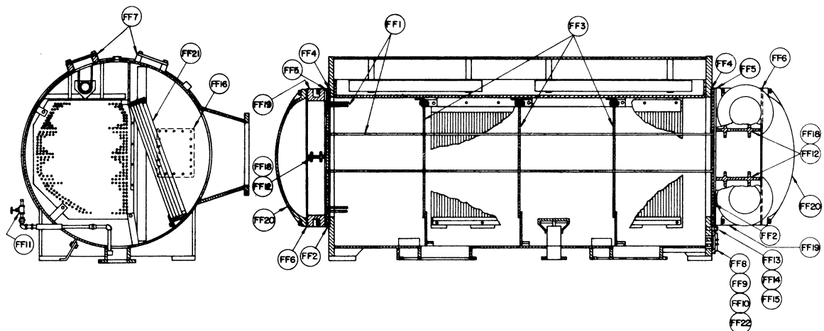
WELDED STEEL COOLER #11 1/2 AND #12 1/2
