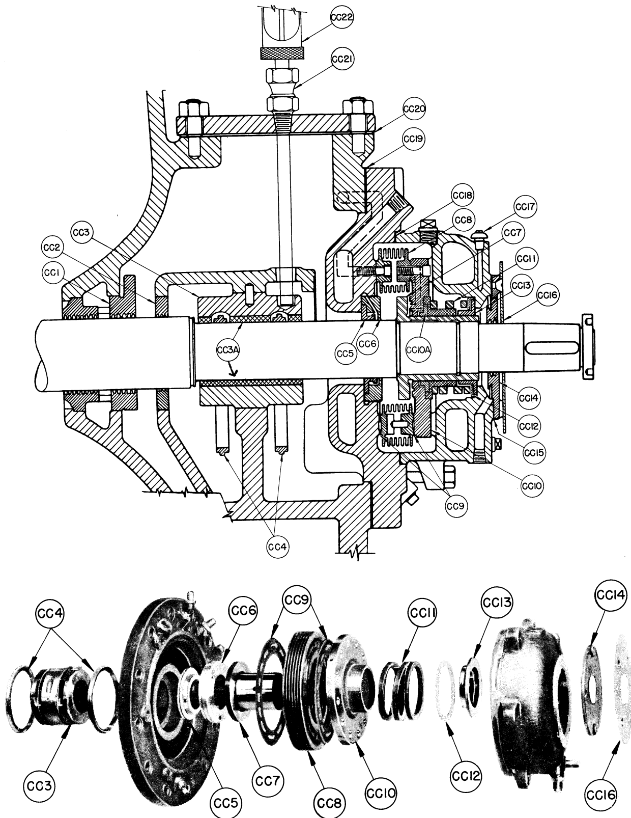
"AA", "BZ", "CZ" AND "DZ" COMPRESSOR SEAL PARTS
