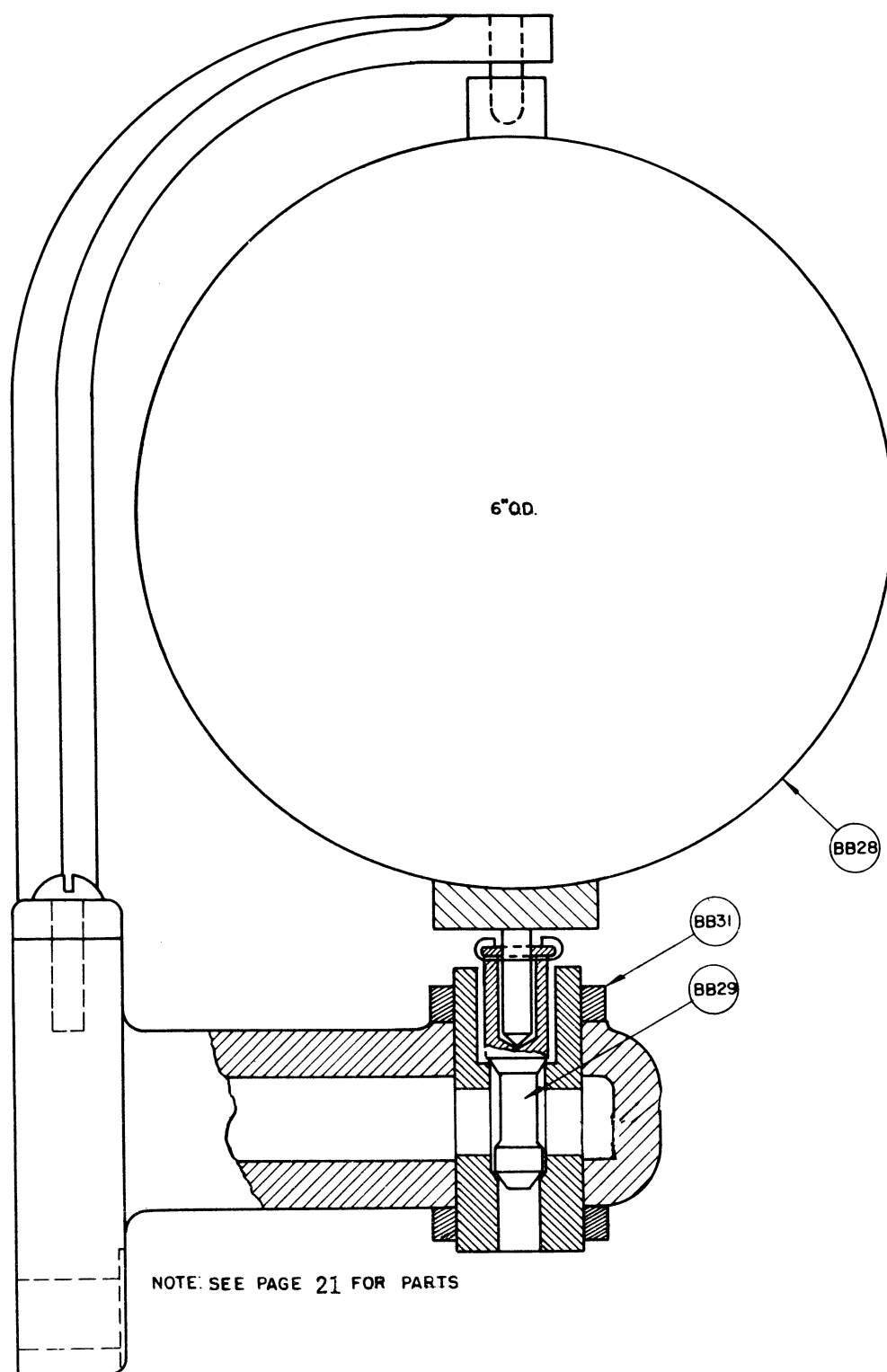
"DZ" ATMOSPHERIC FLOAT VALVE
