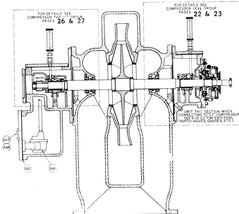
"AA" COMPRESSOR
