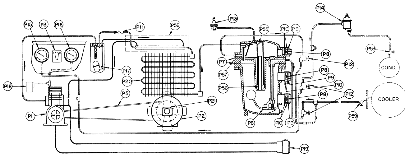
TYPE "L" PURGE UNIT
