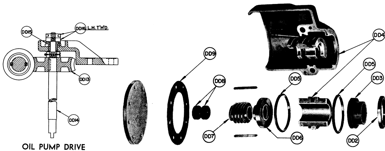
TYPE "AA" AND "BZ" COMPRESSOR THRUST END
