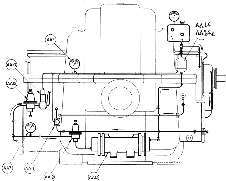
"BZ" COMPRESSOR (EXTERNAL PARTS)
