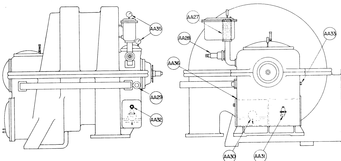
"DZ" COMPRESSOR (EXTERNAL PARTS)
