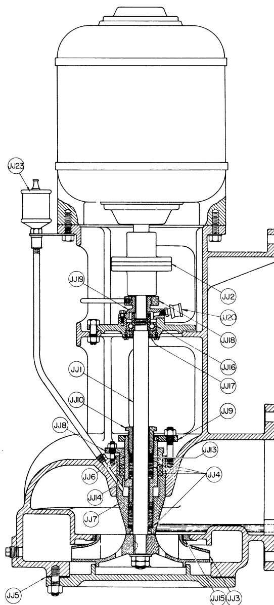
3" AND 4" LIQUID PUMP
