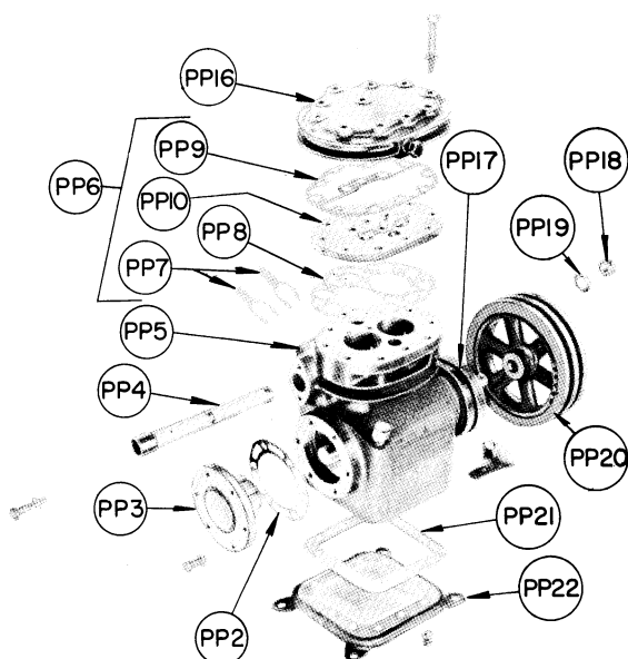
PURGE COMPRESSOR PARTS
