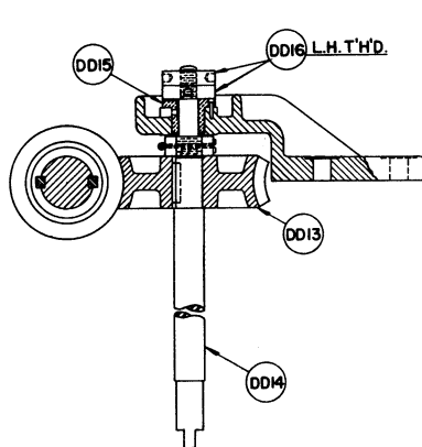
OIL PUMP DRIVE
