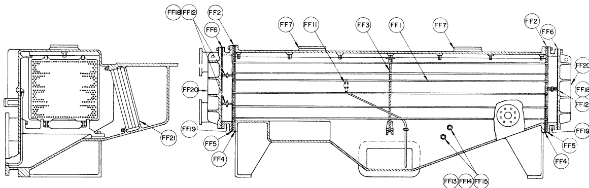
CAST IRON COOLER #7 1/2 THRU #10 1/2
