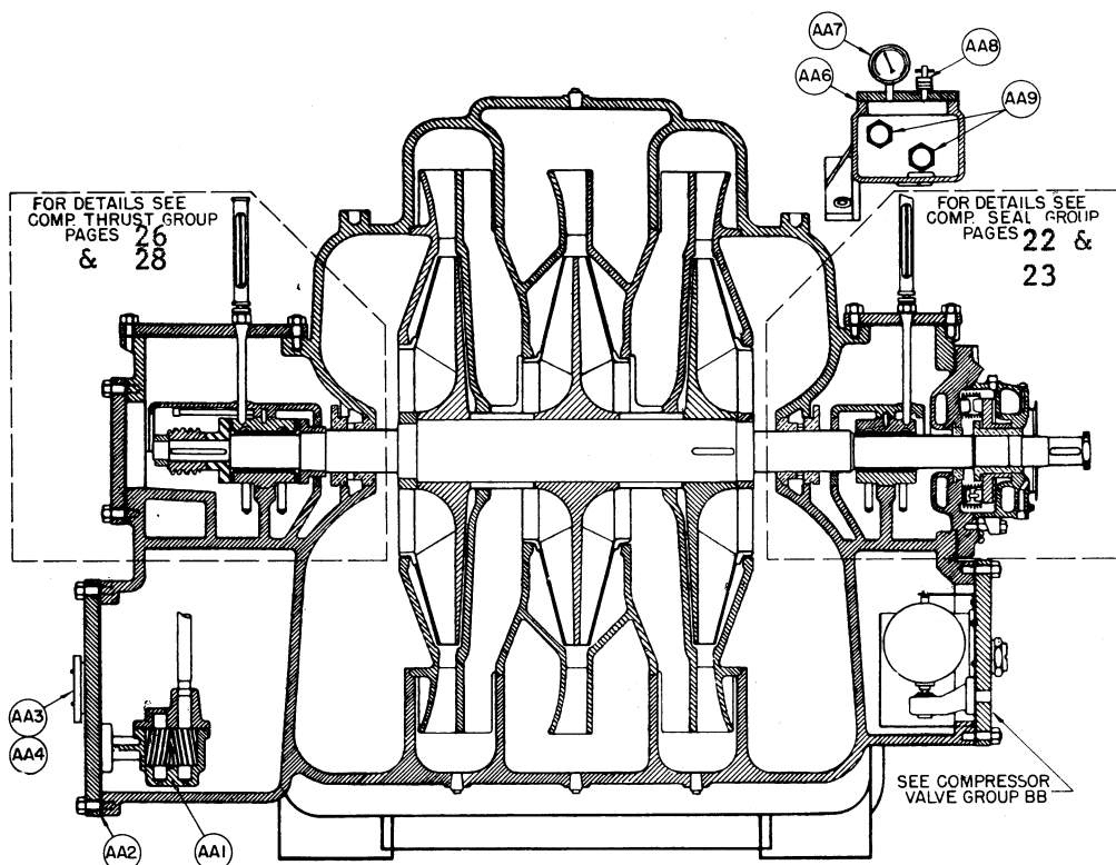
"BZ" COMPRESSOR (INTERNAL PARTS)
