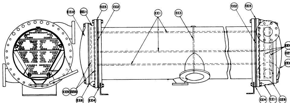
WELDED STEEL CONDENSER #6 1/2
