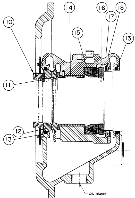
Main Bearing (R-114 Only)
