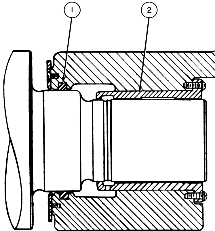
Rear Bearing, Used with R thru XX Motors
