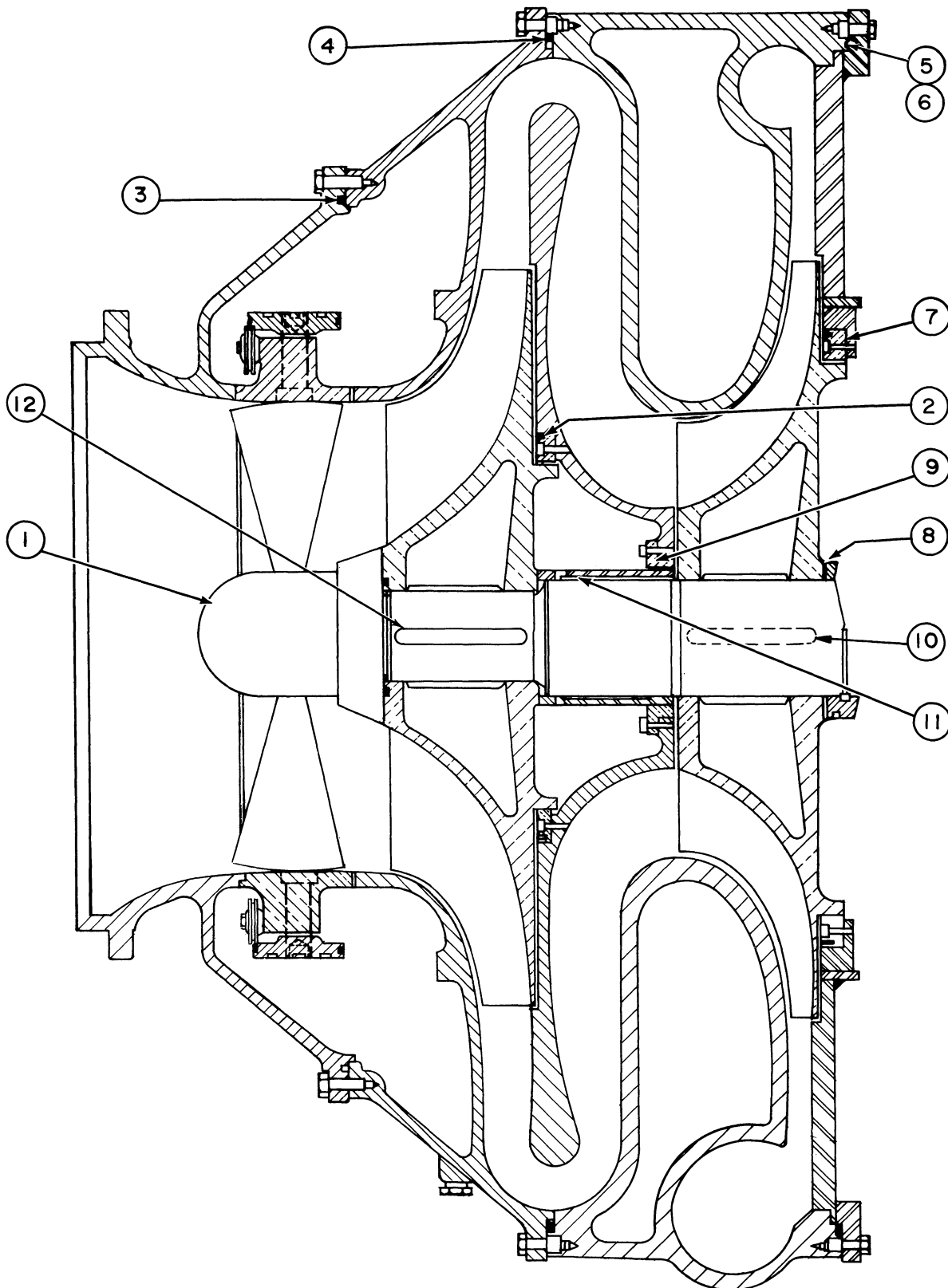
Compressor Assembly
