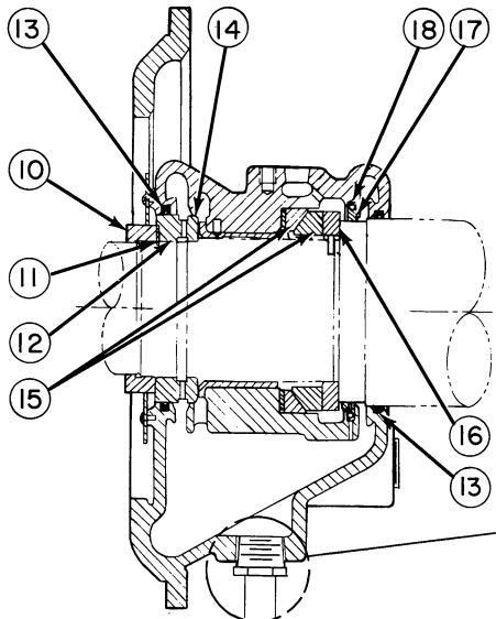
Main Bearing (R-11)
