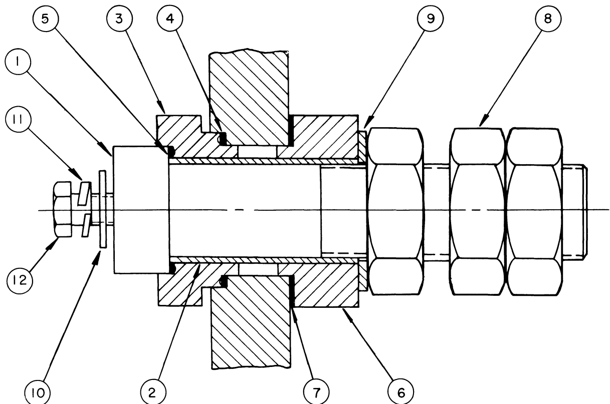
Lo-Voltage Motor Terminals
