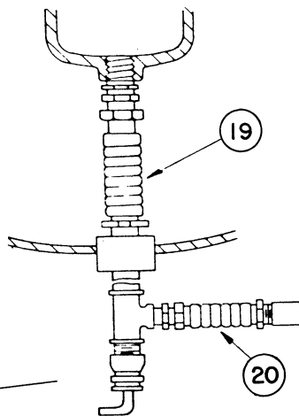
Main Bearing Drain
