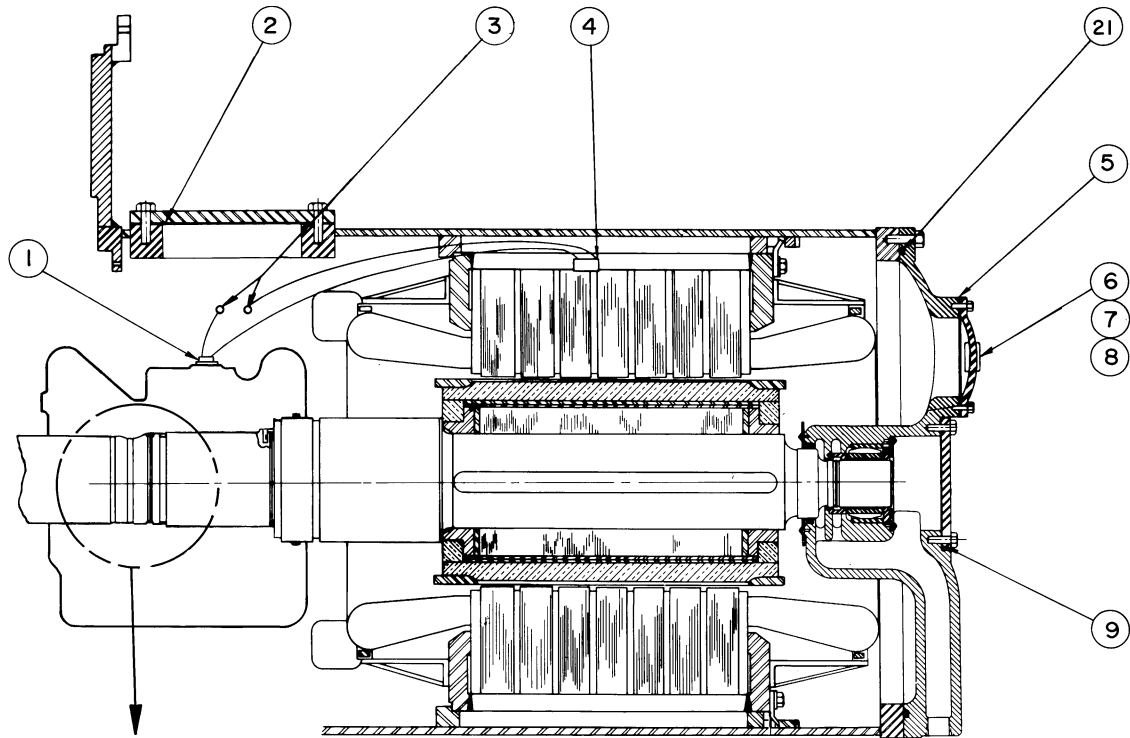
Motor Group
