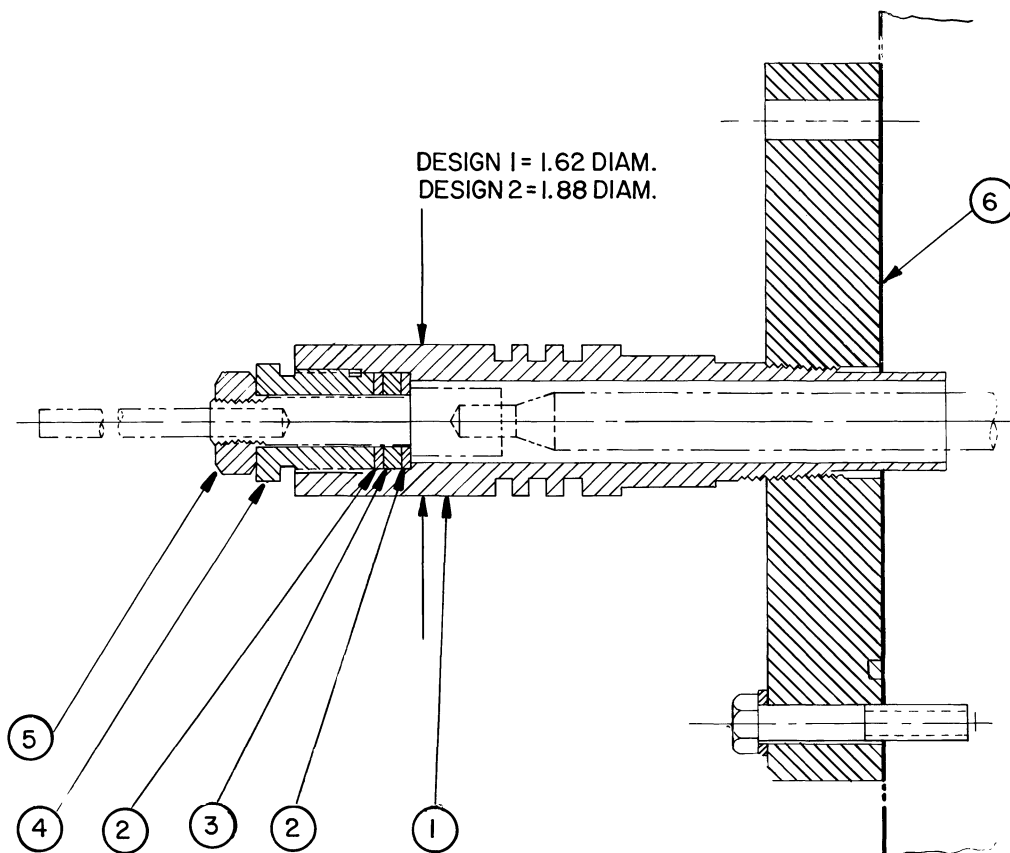
Terminal Arrangement (Hi-Voltage) Used with Motors R thru XX
