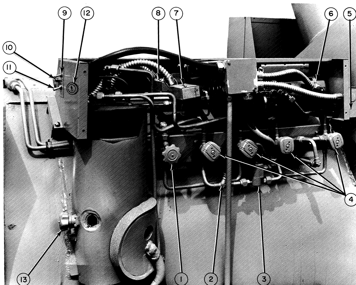
Purge Assembly Controls (R11)
