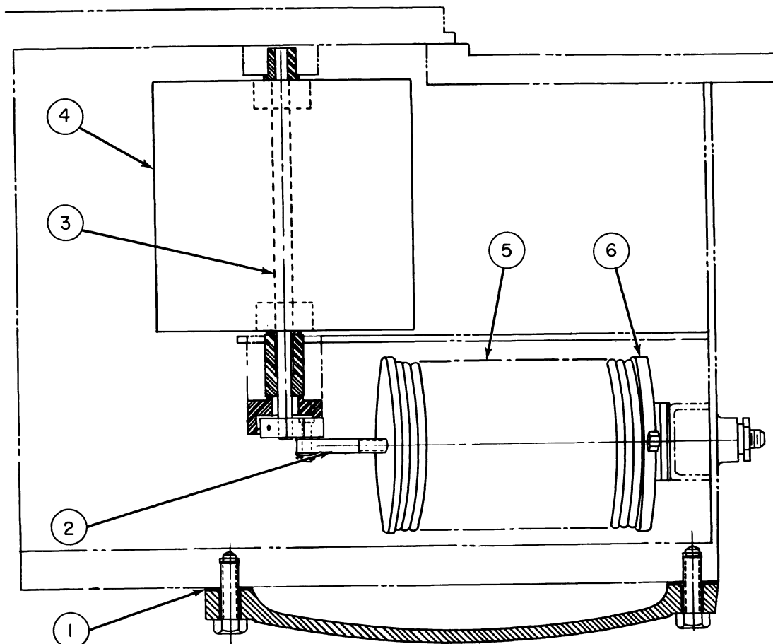
Damper Assembly (R-114 Only)
