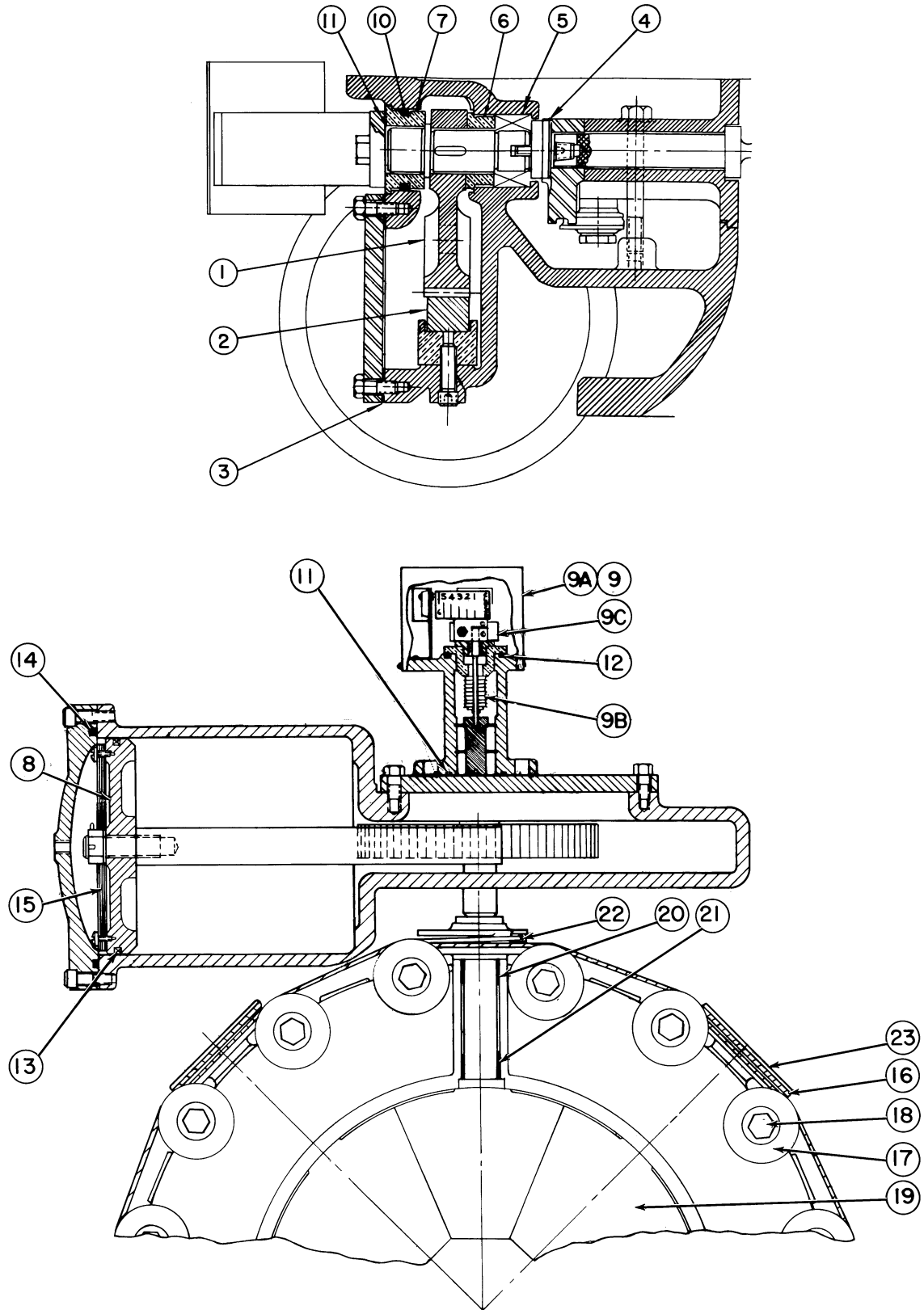
Inlet Venturi Hydraulic-Electronic
