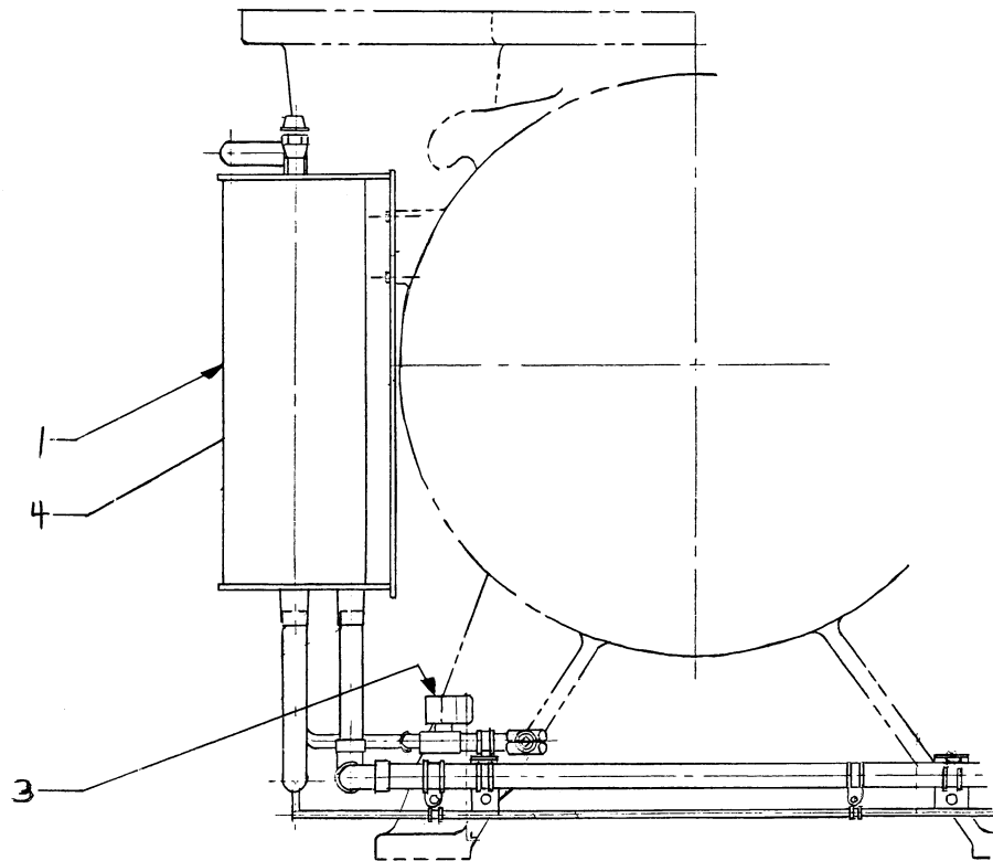
Oil Lube System
