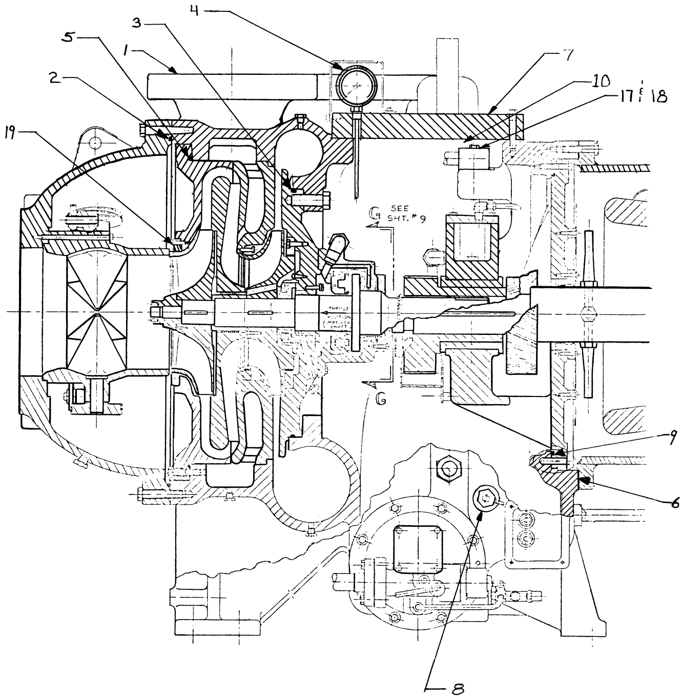
Compressor Drive Train
