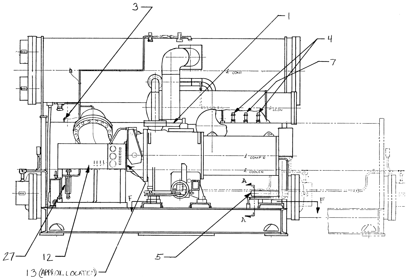
Refrigeration Machine Assembly
