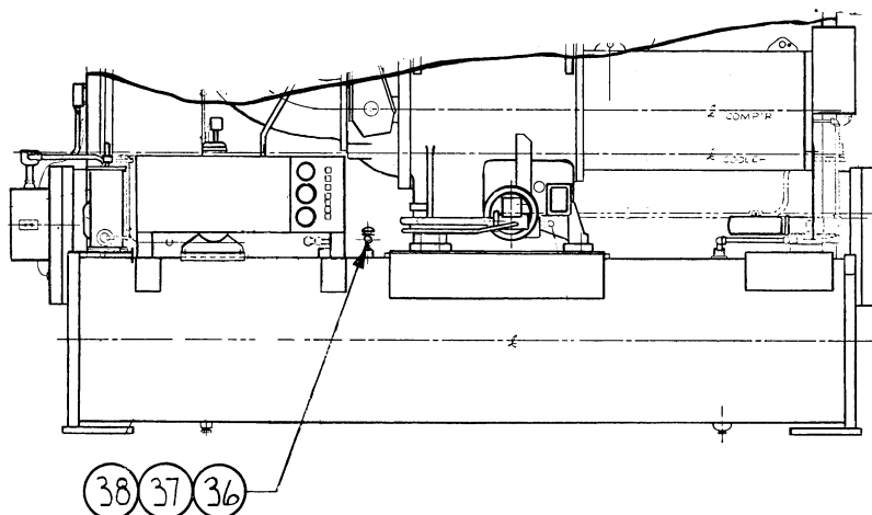
FRONT VIEW / w STORAGE TANK
