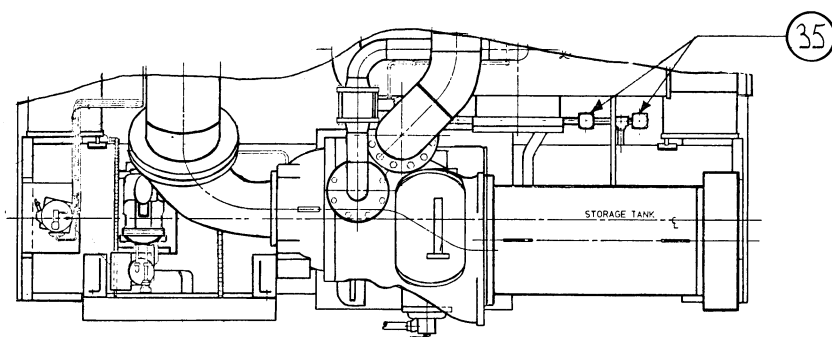
PLAN VIEW / w STORAGE TANK
