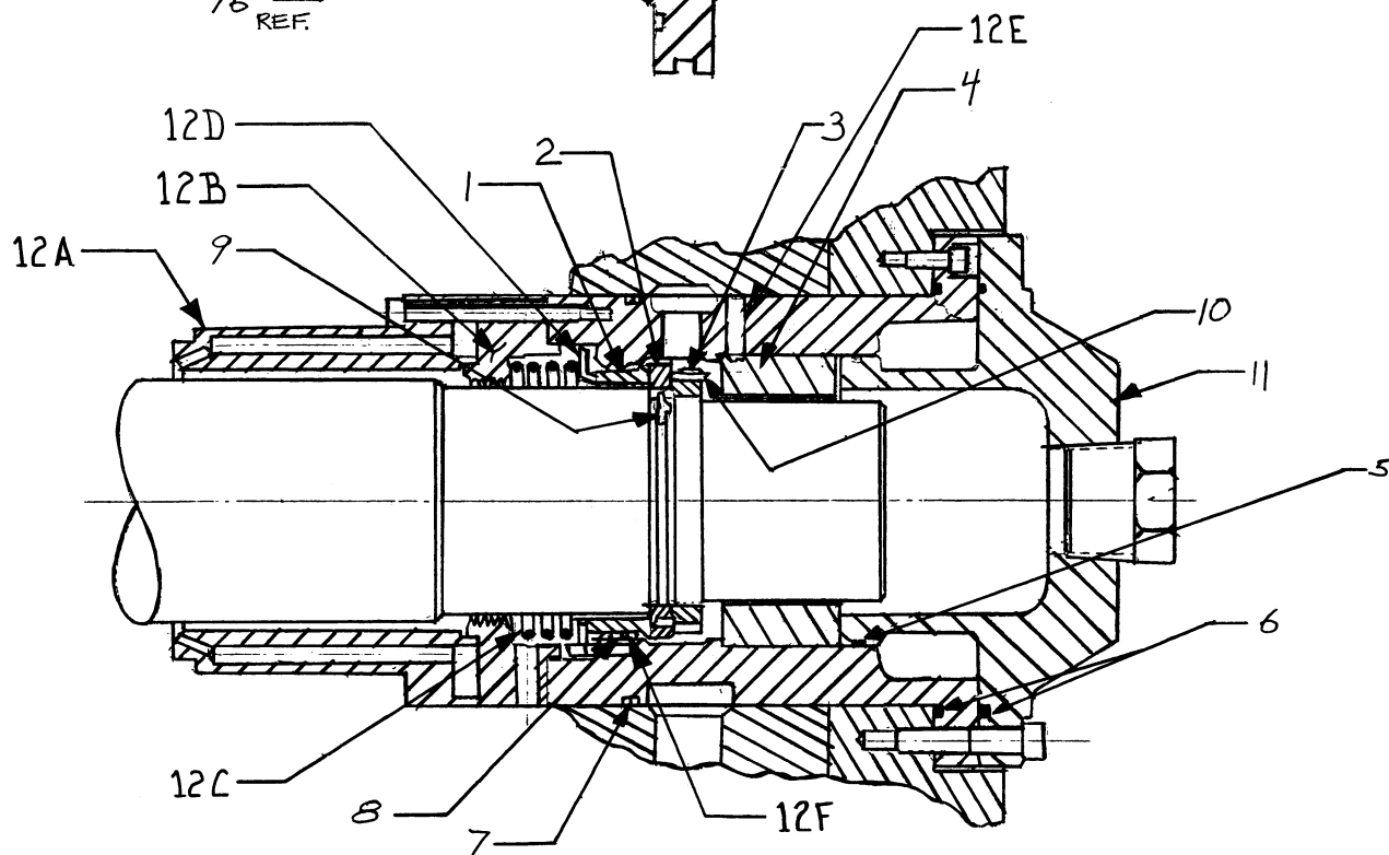
Compressor Rear Bearing Assembly
