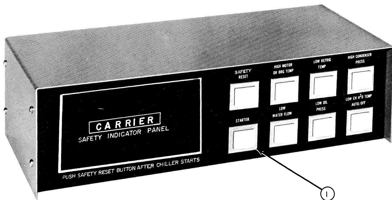
Safety Indicator Panel
