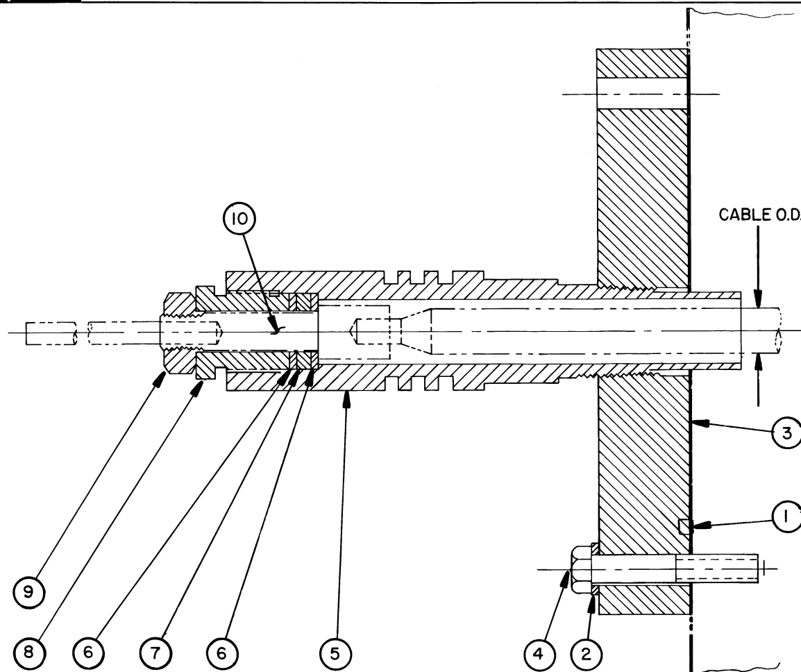
Terminal Arrangement (Hi-Voltage, 2300-4160)
