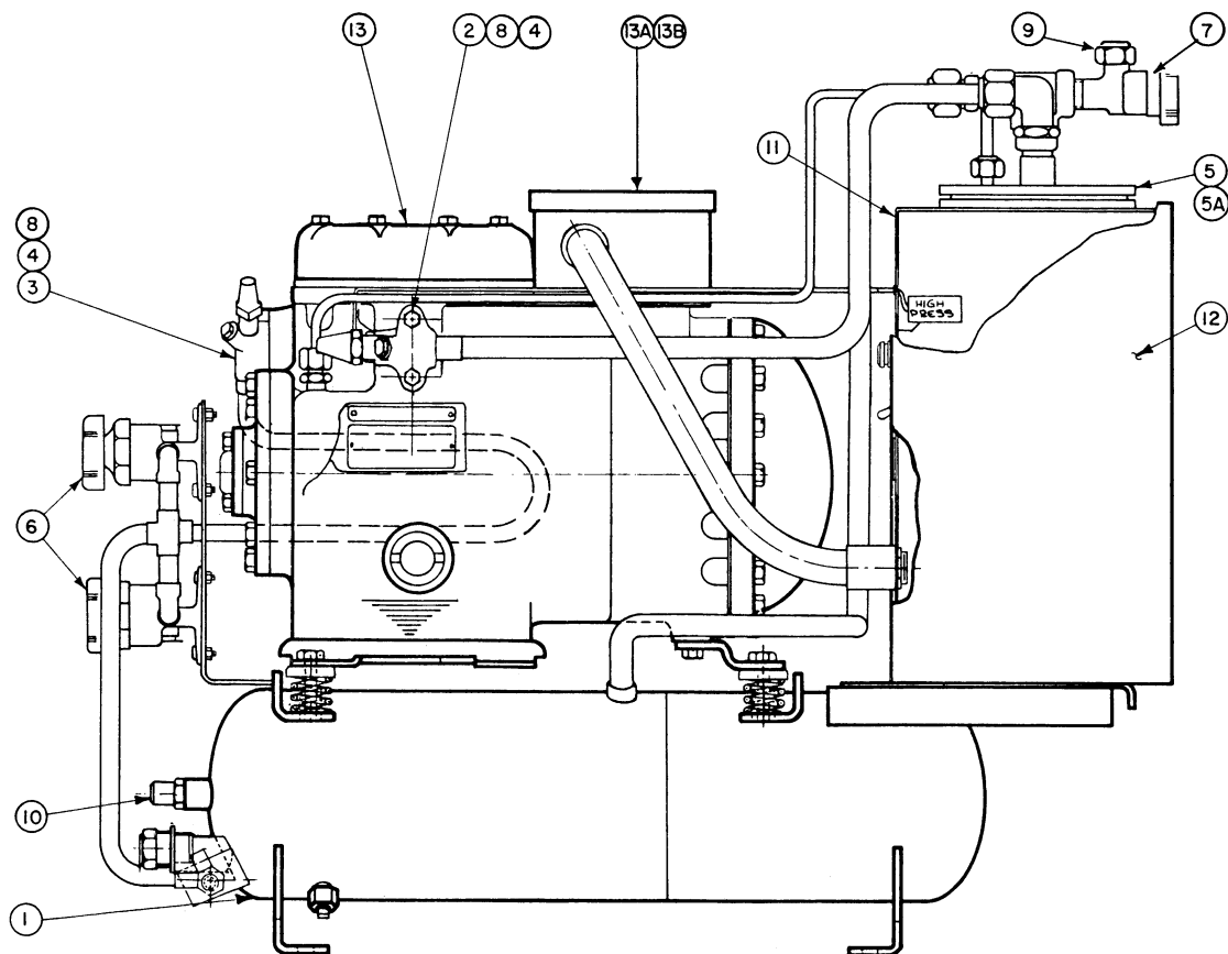
Pumpdown Assembly
