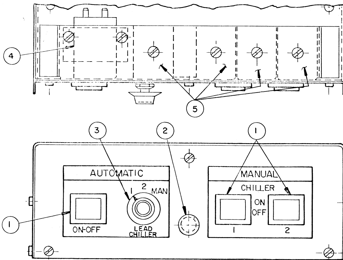
LEAD - LAG CONTROL ASSEMBLY (32SM-900---001--)
