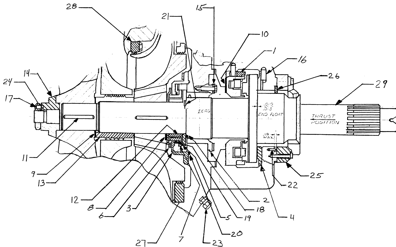
Rotor Bearing Assembly
