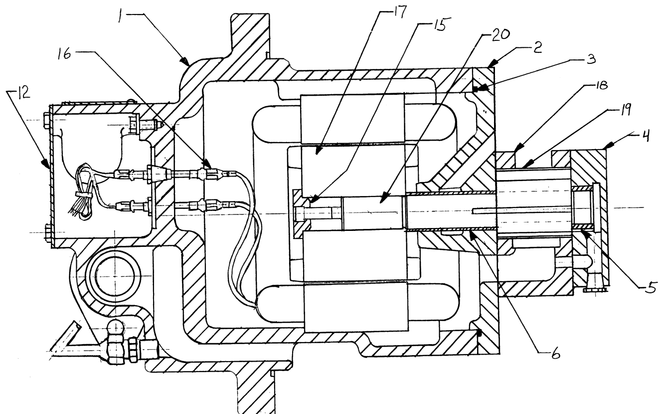
Oil Pump and Motor Assembly
