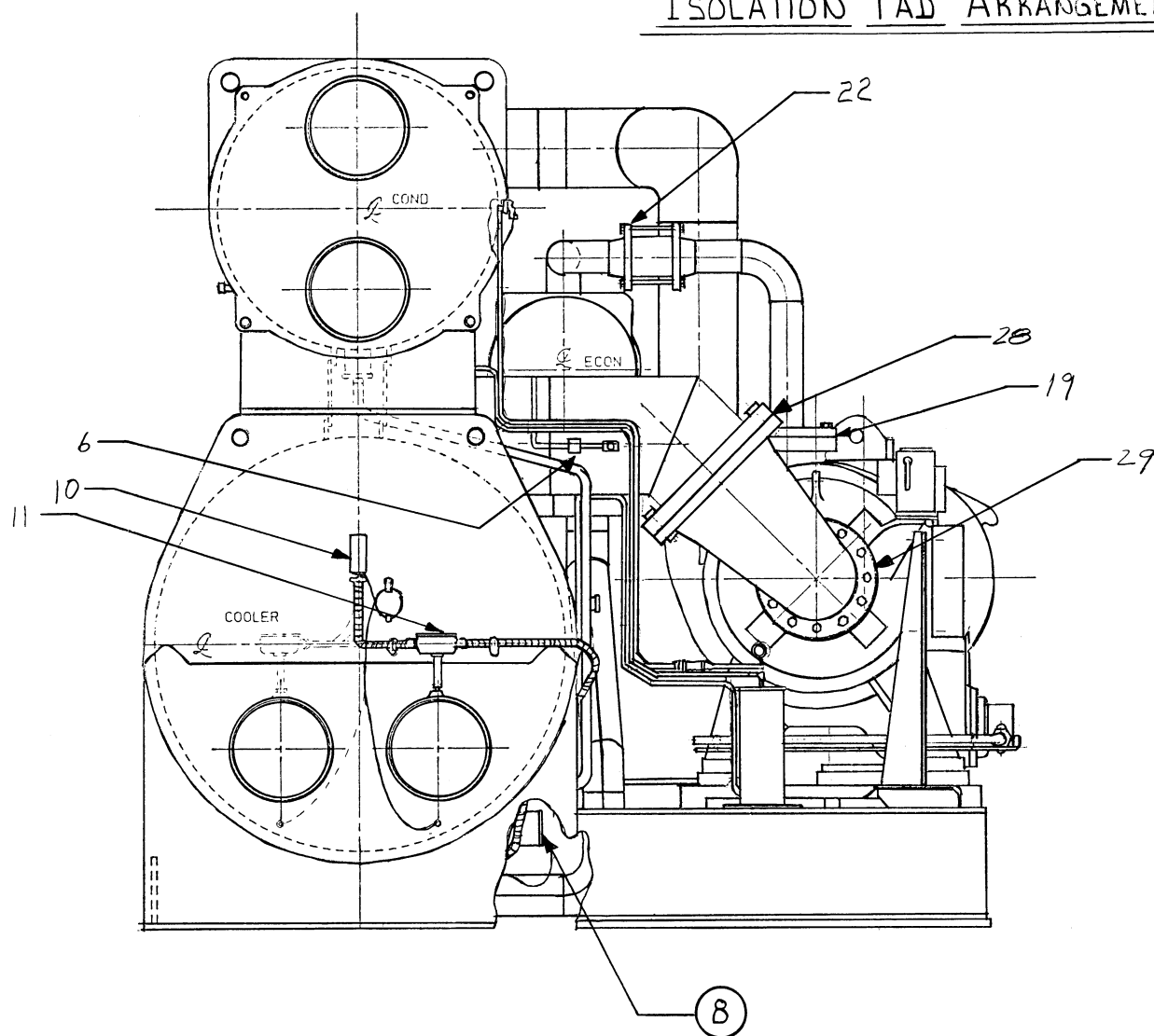
ISOLATION PAD ARRANGEMENT
