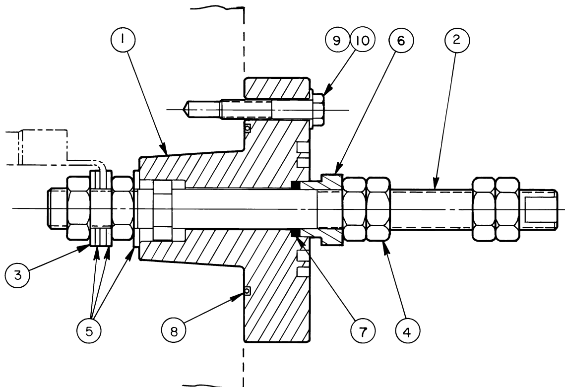
Terminal Arrangement (Lo-Voltage, 208-575)
