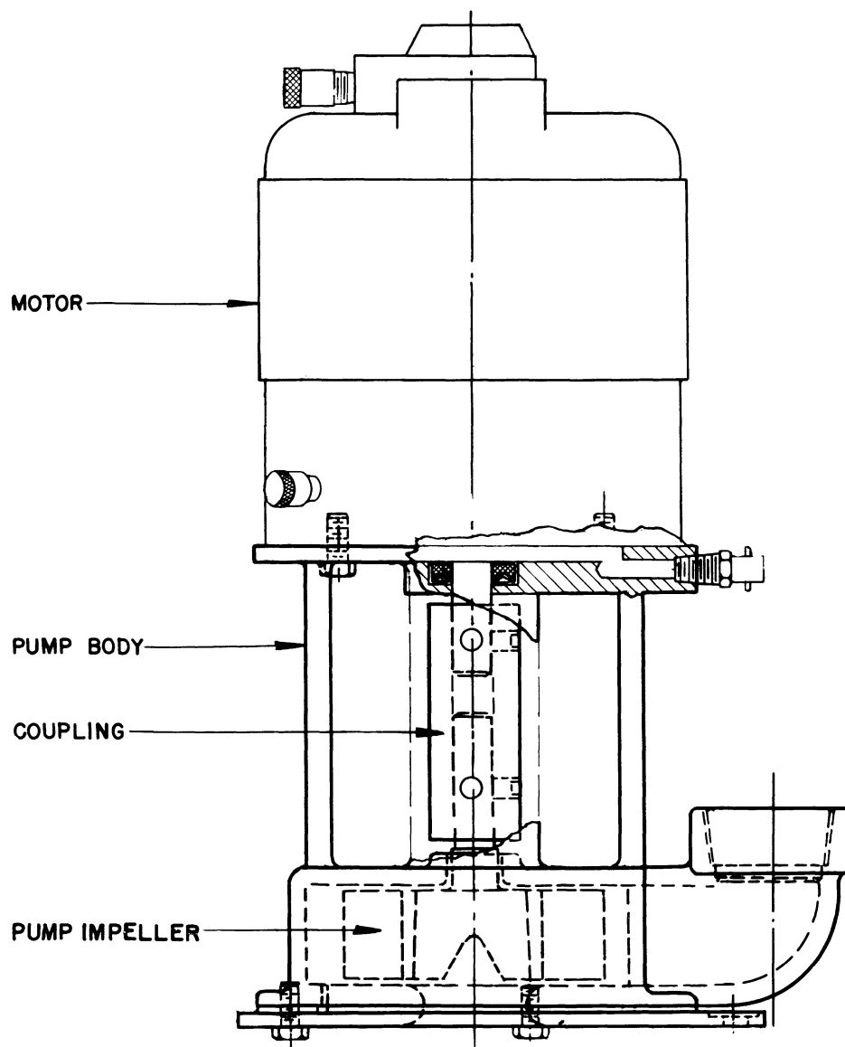
23C PUMP AND MOTOR ASSEMBLY
