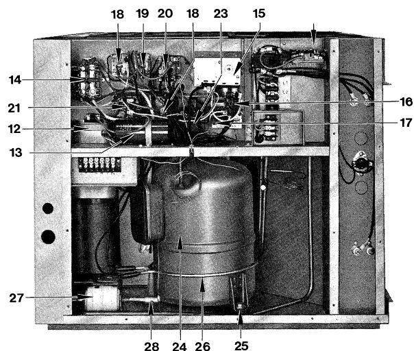
COMPRESSOR & CONTROL COMPARTMENT
