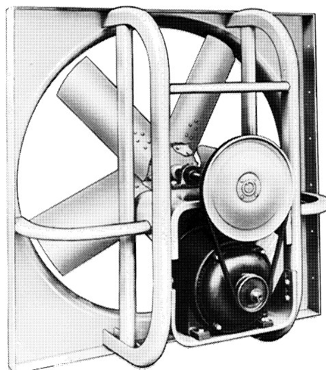
27FD - Belt Drive Industrial Propeller Fan
