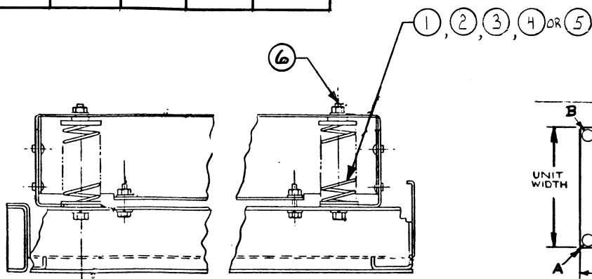
TYPICAL ISOLATOR ASSEMBLY
