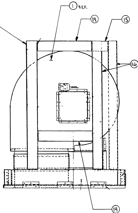
SIDE VIEW- DBF, DBR
