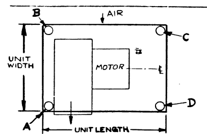
ISOLATOR ARRANGEMENT NOTE: "A" IS ALWAYS AT DISCHARGE END, ADJACENT TO SCROLL
