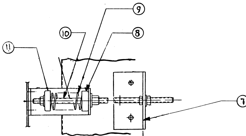
SNUBBER MOUNT
