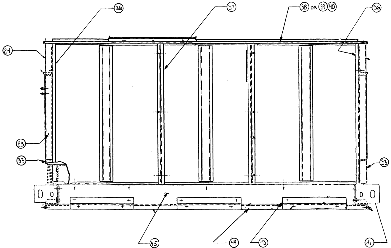
DOWNBLAST FRONT 60/70 SIZE
