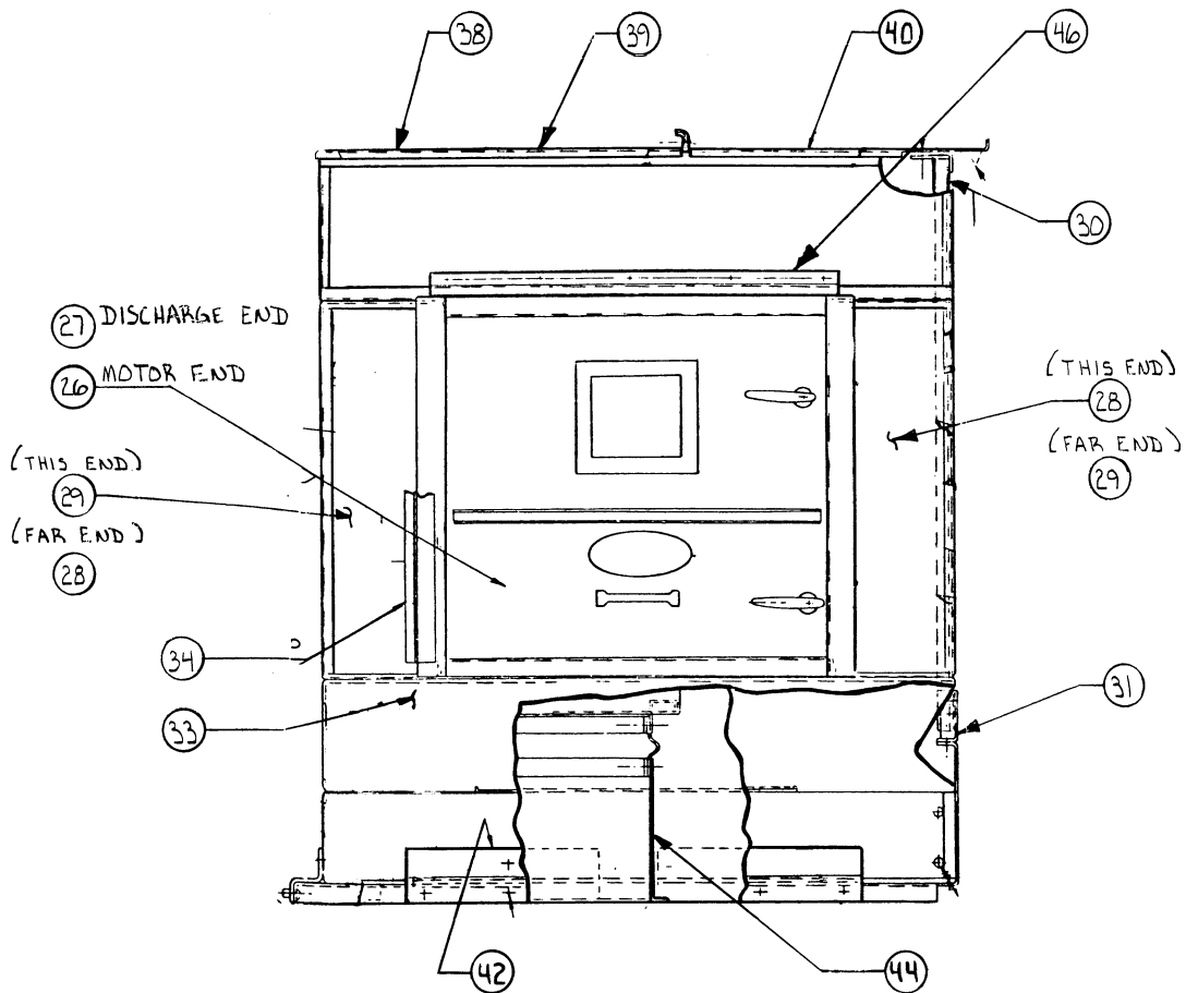
DOWNBLAST FRONT 60/70 SIZE
