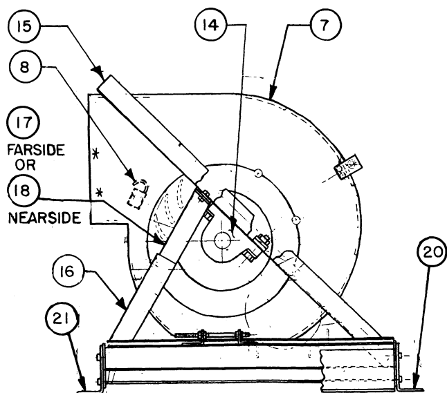
DRIVE END
