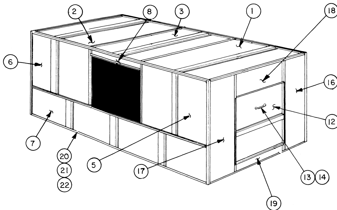
TYPICAL FOR 39E — FAN SECTION PANELS FAN DOOR BOLTED (48 AND 57 SIZE UNIT) (DESIGN #1, S/N 7825XXXXX AND LOWER)
