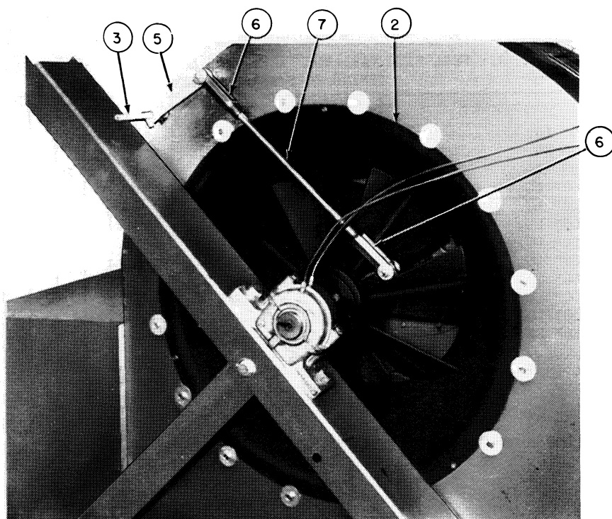
AIRFOIL WITH INLET GUIDE VANE
