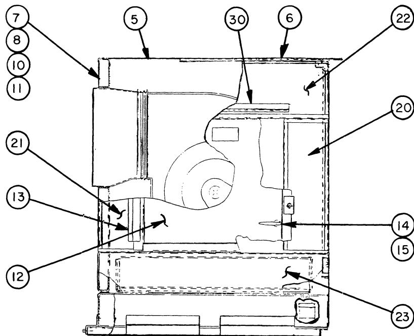
VIEW S-S
