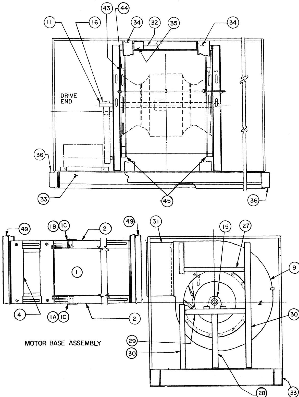
TYPICAL FOR 39E — A.F. INTERNAL FAN SECTION (NON-ISOLATED) 75 AND 90 SIZE UNIT (PRIOR TO S/N 1684XXXXX)
