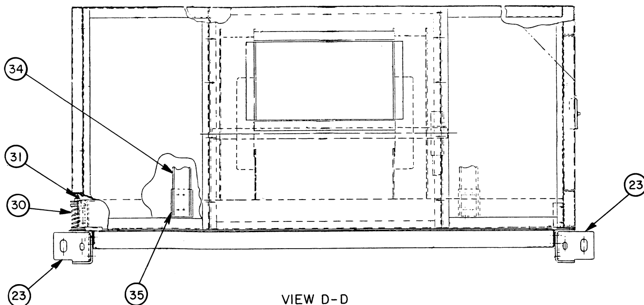
TYPICAL FOR 39E — F.C. INTERNAL FAN SECTION WITH INLET GUIDE VANES (VIV) (ISOLATED) 08-57 SIZE UNIT (START S/N 4785XXXXXX AND HIGHER)
