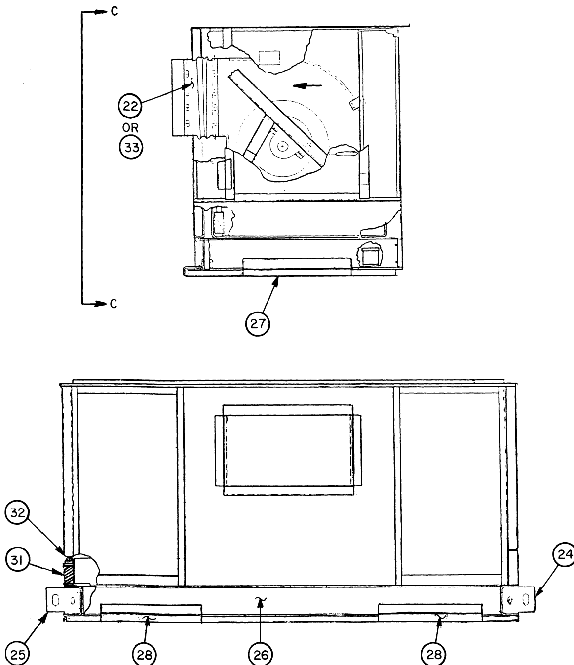
VIEW C-C
