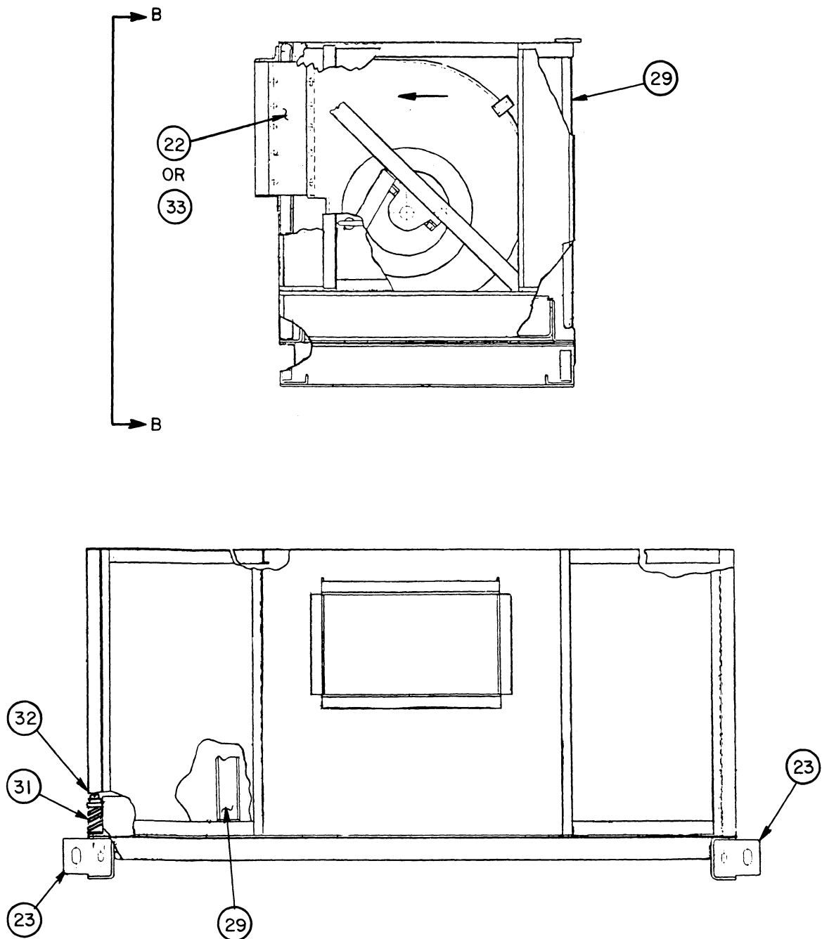
VIEW B-B
