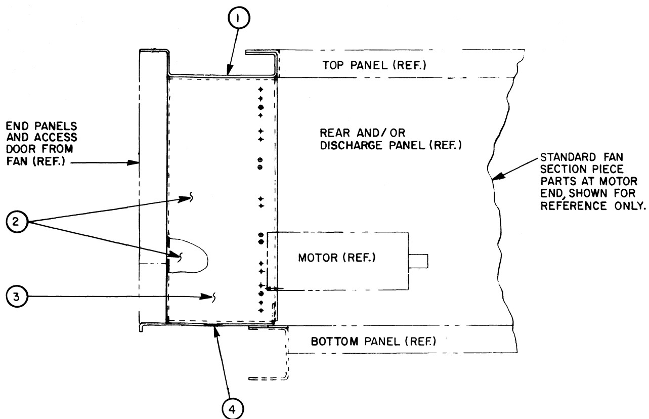
LARGE MOTOR EXTENSION PANEL
