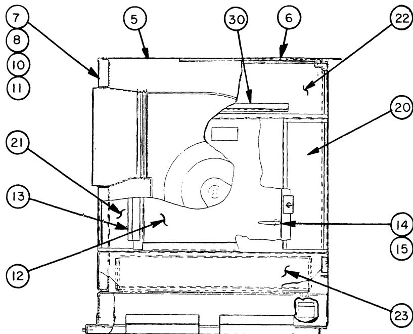
VIEW S-S
