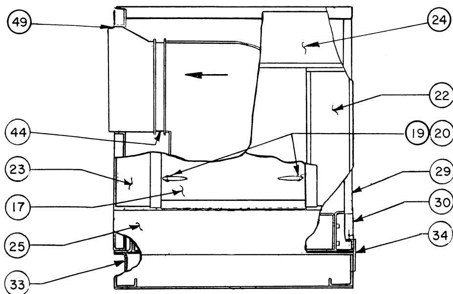
VIEW H-H
