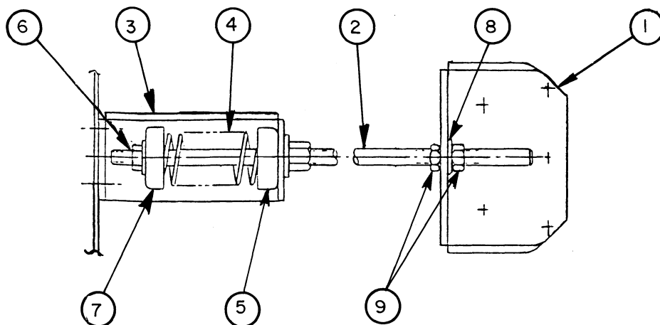
08 - 90 SIZE UNIT (PRIOR TO S/N 1684XXXXX)
