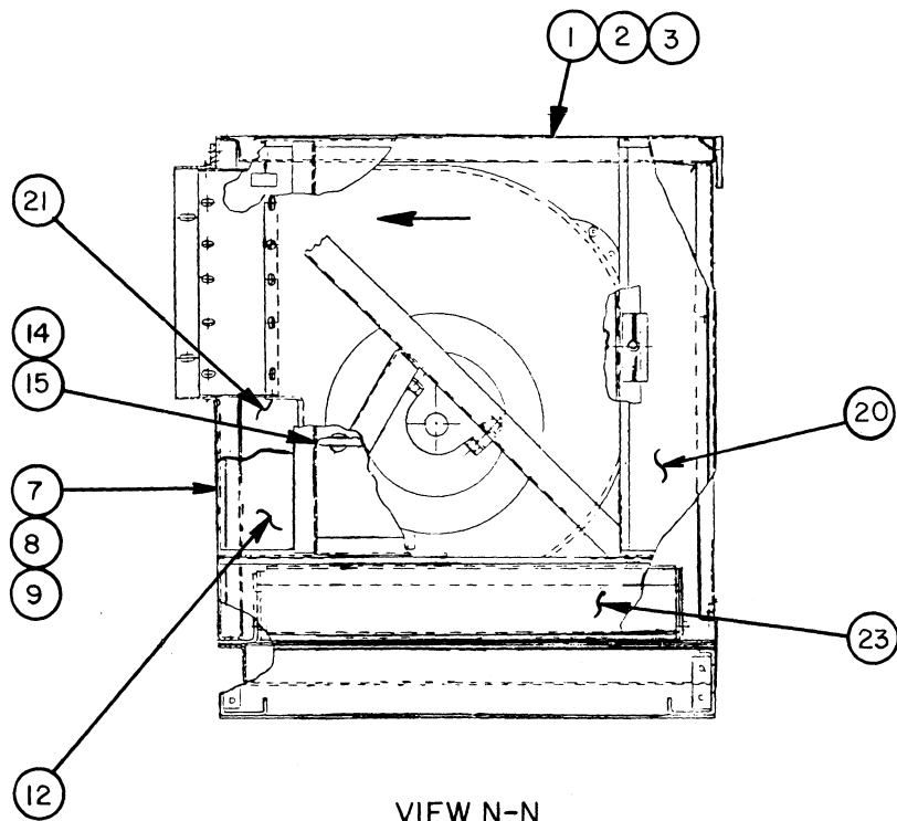
VIEW N-N
