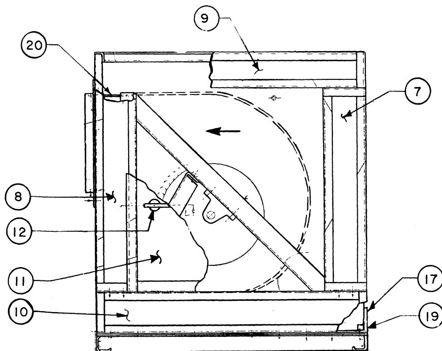
VIEW M-M
