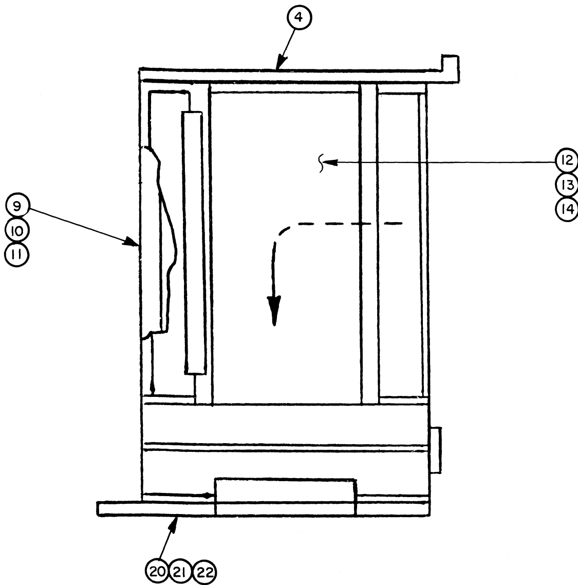
TYPICAL FOR 39ER ROOFTOP FAN SECTION PANELS DOWN BLAST (MOTOR END) (S.F.A.N.) (DESIGN #1, S/N 7825XXXXX AND LOWER)
