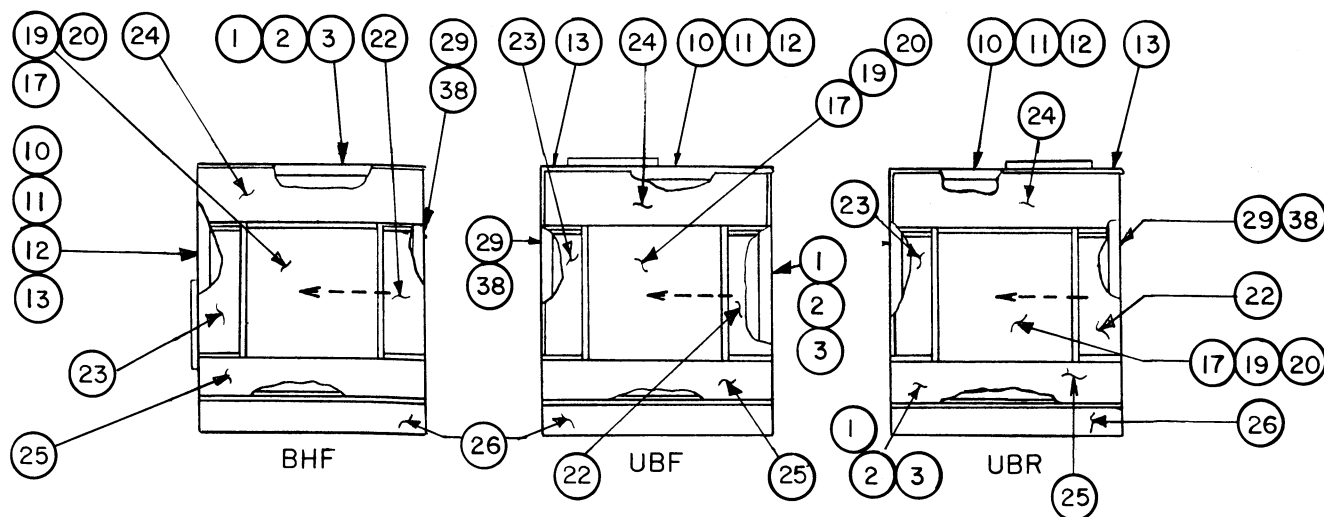
39E — INDOOR UNIT ARRANGEMENTS
