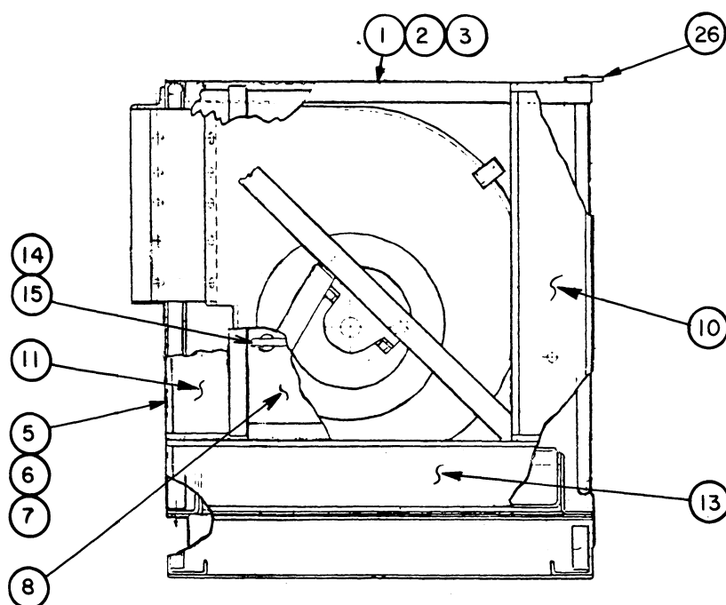
VIEW K-K
