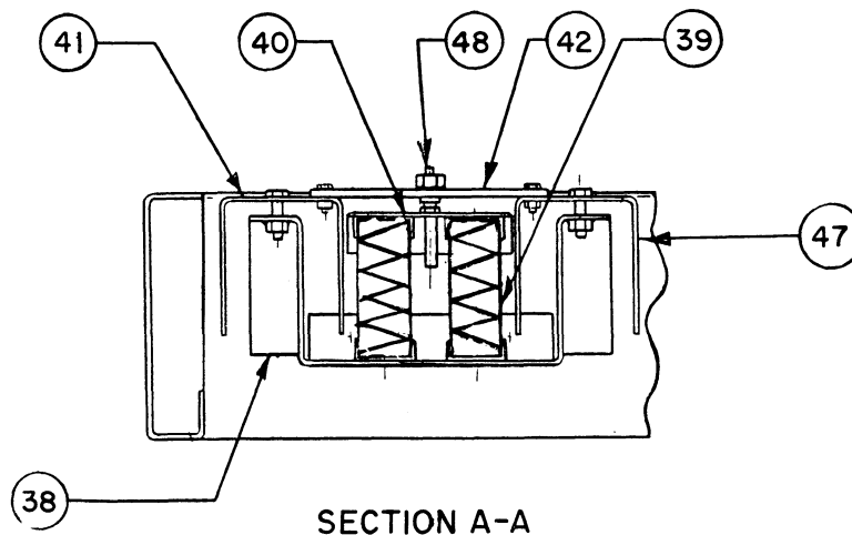
TYPICAL FOR 39E — A.F. INTERNAL FAN SECTION BASE ASSEMBLY (ISOLATED) 75 AND 90 SIZE UNIT (PRIOR TO S/N 1684XXXXX)
