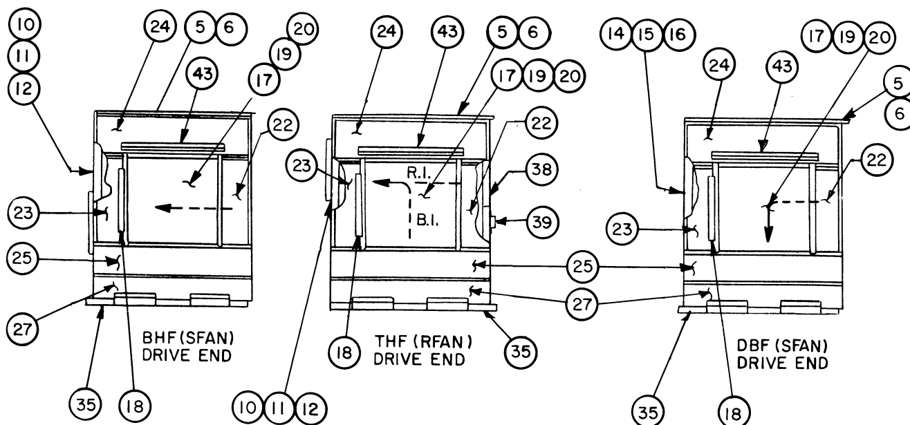
39ER ROOFTOP UNIT ARRANGEMENTS
