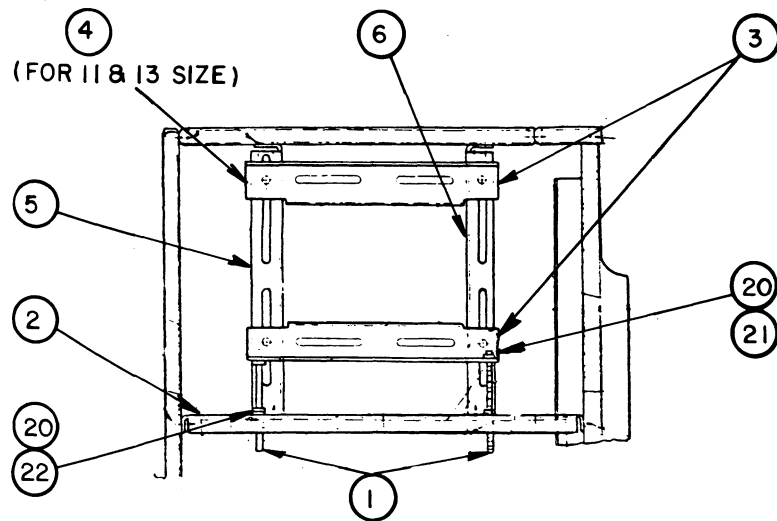
MOTOR BASE ASSEMBLY (B.H.F. & U.B.R.) L.H. UNIT
