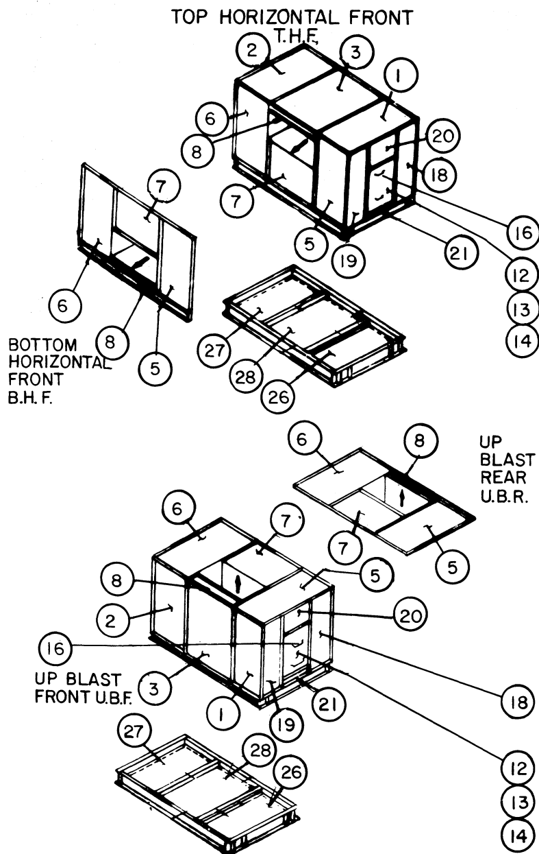
TYPICAL FOR 39E — FAN SECTION PANELS FAN POOR WING NUTS (75 AND 90 SIZE UNITS) (DESIGN #2, S/N 7826XXXXX AND HIGHER)
