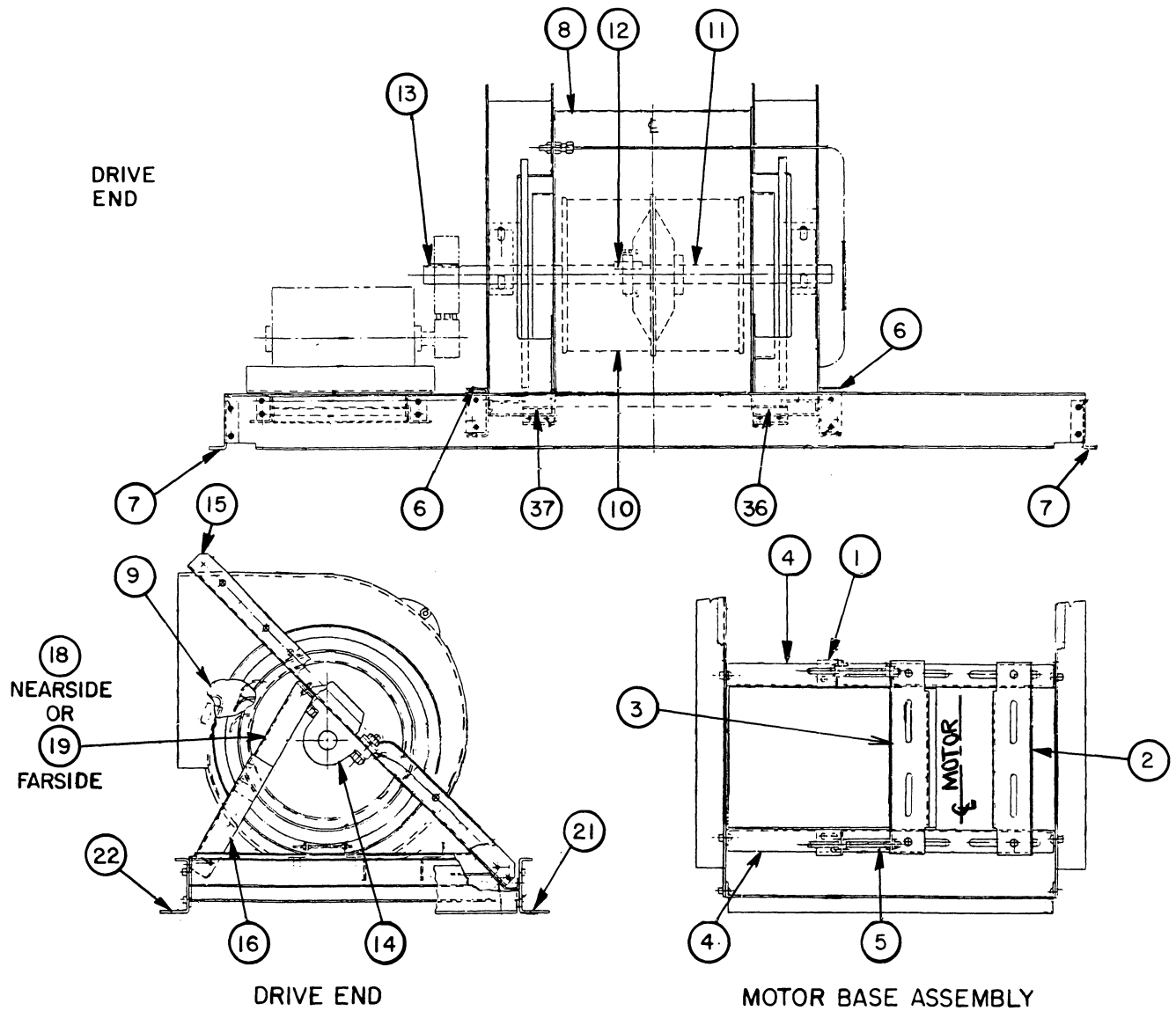
TYPICAL FOR 39E — F.C. INTERNAL FAN SECTION WITH INLET GUIDE VANES (IVV) 08-57 SIZE UNIT (START S/N 4785XXXXX AND HIGHER)
