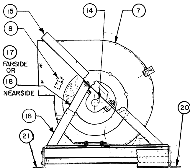
DRIVE END
