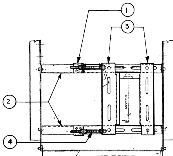
MOTOR BASE ASSEMBLY
