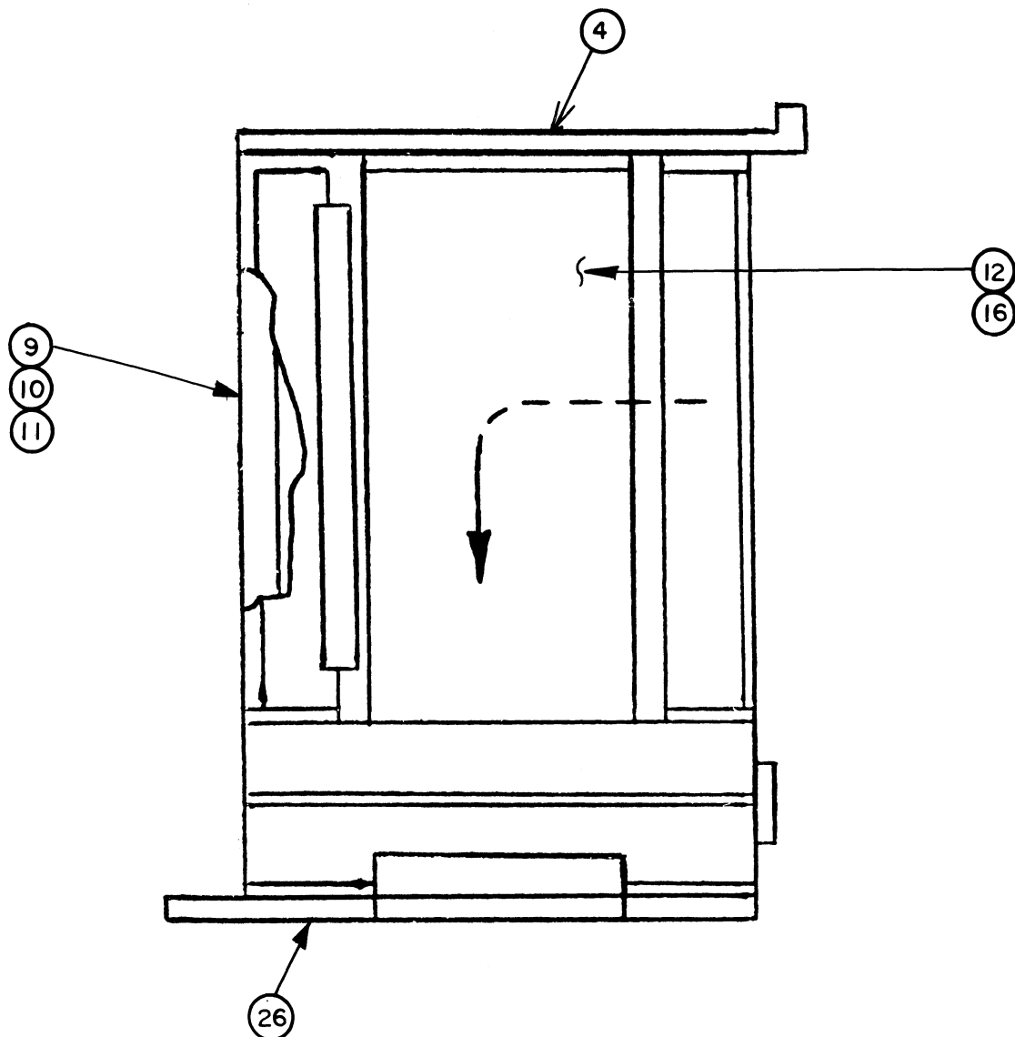
TYPICAL FOR 39ER ROOFTOP FAN SECTION PANELS DOWN BLAST (MOTOR END) (S.F.A.N.) (DESIGN #2, S/N 7826XXXXX AND HIGHER)
