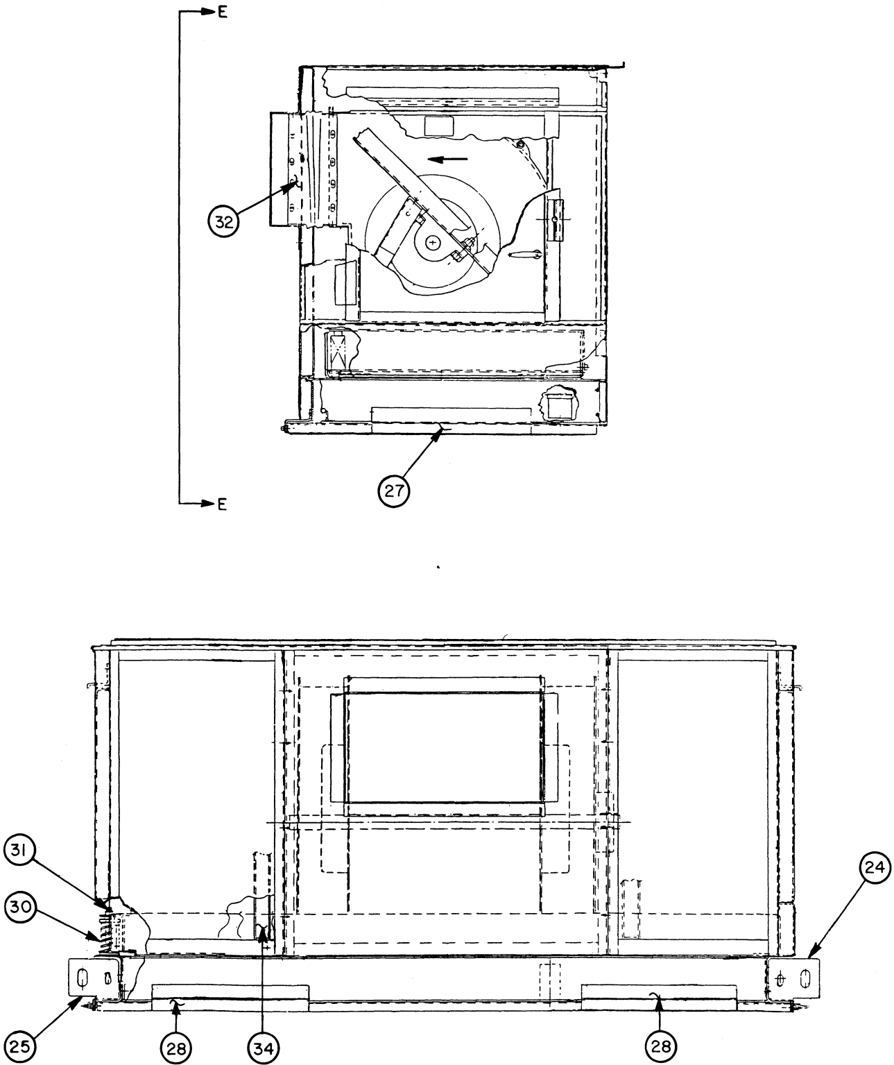
VIEW E-E
