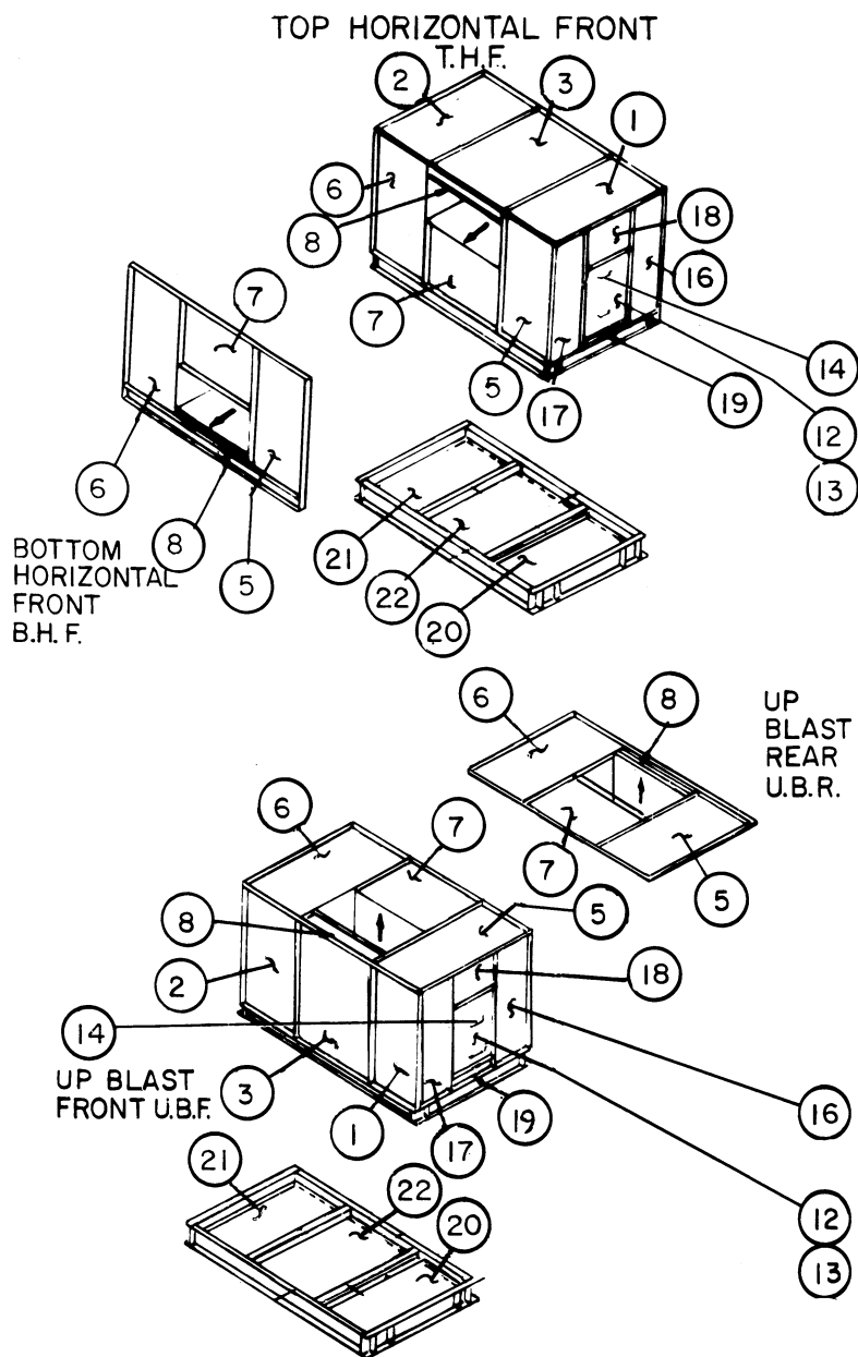
TYPICAL FOR 39E — FAN SECTION PANELS FAN DOOR BOLTED (75 AND 90 SIZE UNIT, (DESIGN #1, S/N 7825XXXXX AND LOWER)
