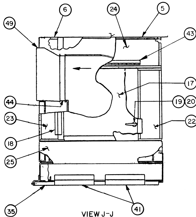
TYPICAL FOR 39ER ROOFTOP FAN SECTION PANELS FAN DOOR WITH LATCH HANDLE T.H.F. (S.F.A.N.) (48 AND 57 SIZE UNIT) (DESIGN #3, S/N 8001XXXXX AND HIGHER)
