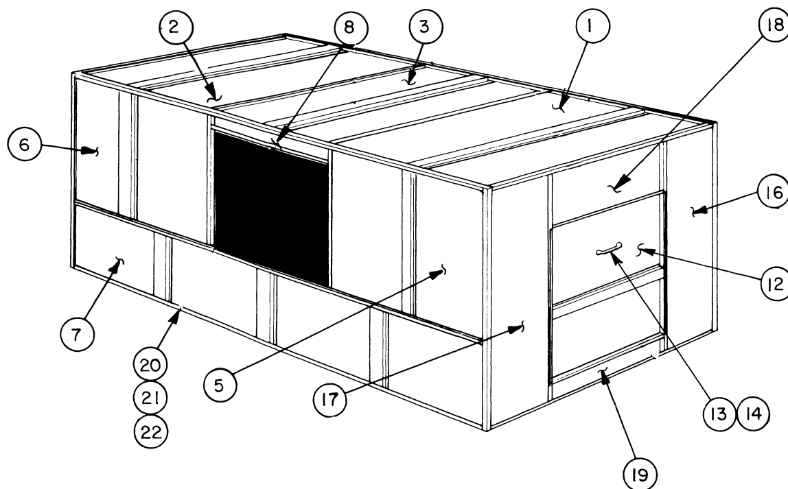
TYPICAL FOR 39E — FAN SECTION PANELS FAN DOOR BOLTED (48 AND 57 SIZE UNIT) (DESIGN #1, S/N 7825XXXXX AND LOWER)
