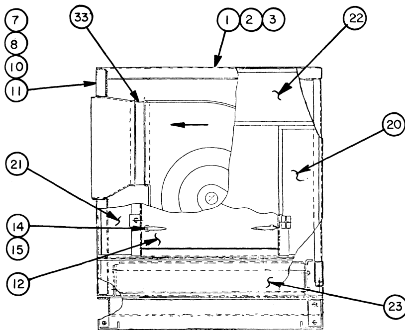
VIEW P-P
