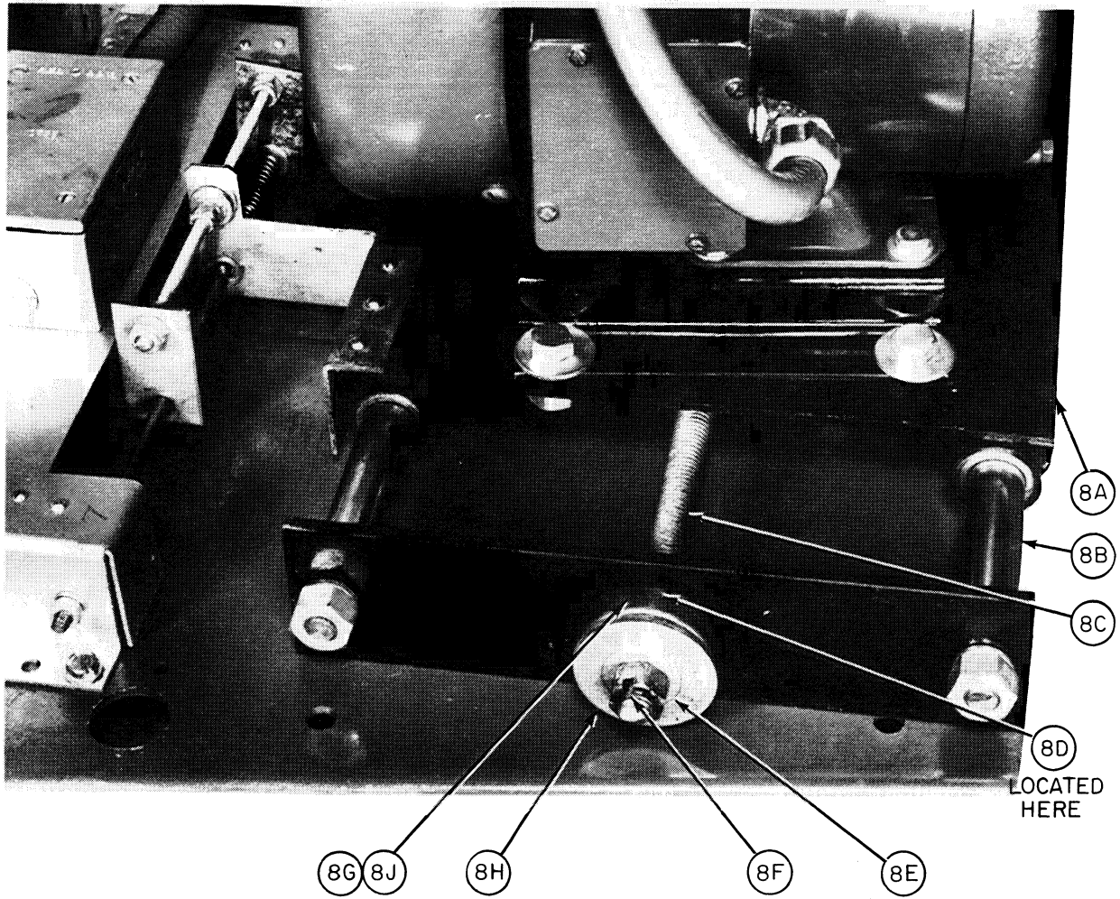
VARIABLE DRIVE BASE ASSEMBLY
