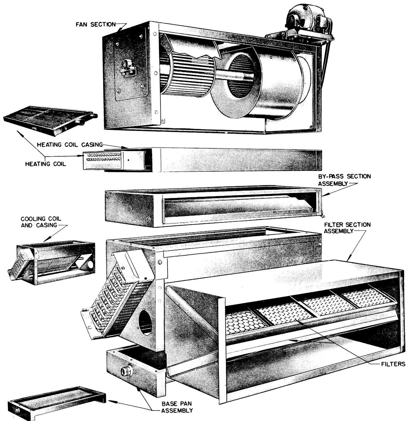
MODEL 39S VERTICAL SYSTEM WEATHERMAKER
