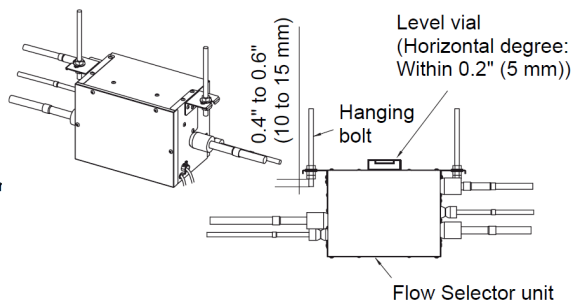
<RBM-Y0383FUL, RBM-Y0613FUL>
