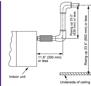
2x2 Cassette
