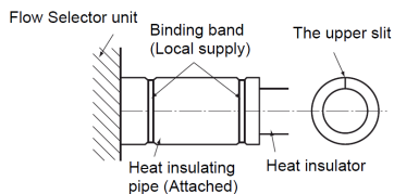
<RBM-Y0383FUL, RBM-Y0613FUL>
