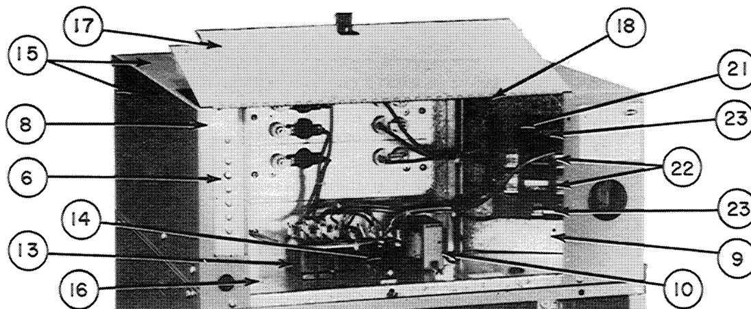
Typical Encased Electric Heater Package (Item 1)
