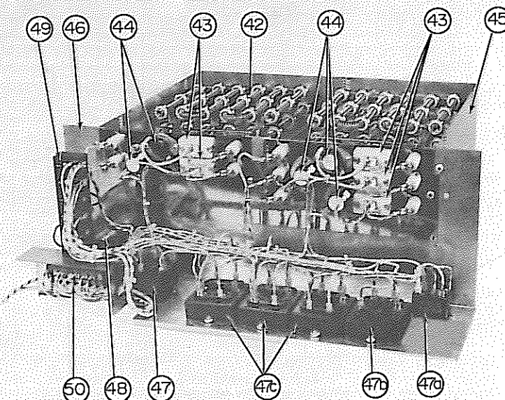
Typical 40VU900081 Electric Heater Package
