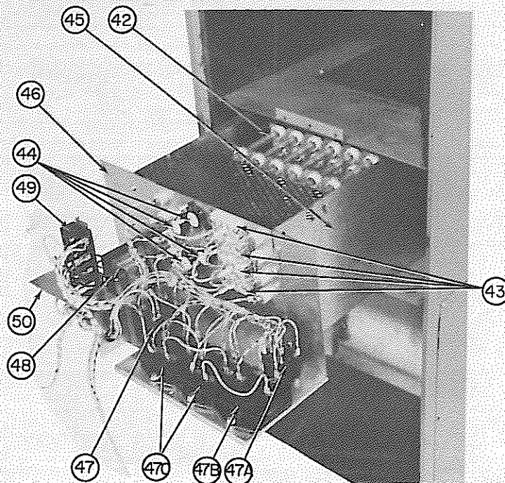
Typical 40VU900051 Electric Heater Package
