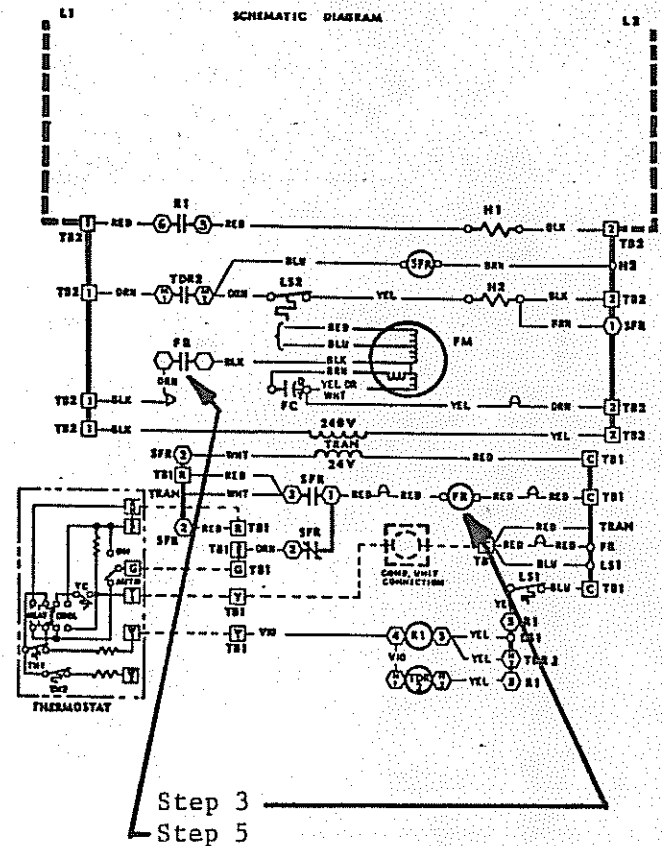
DIAGRAM B Typical wiring diagram showing 3 speed motor in circuit.
